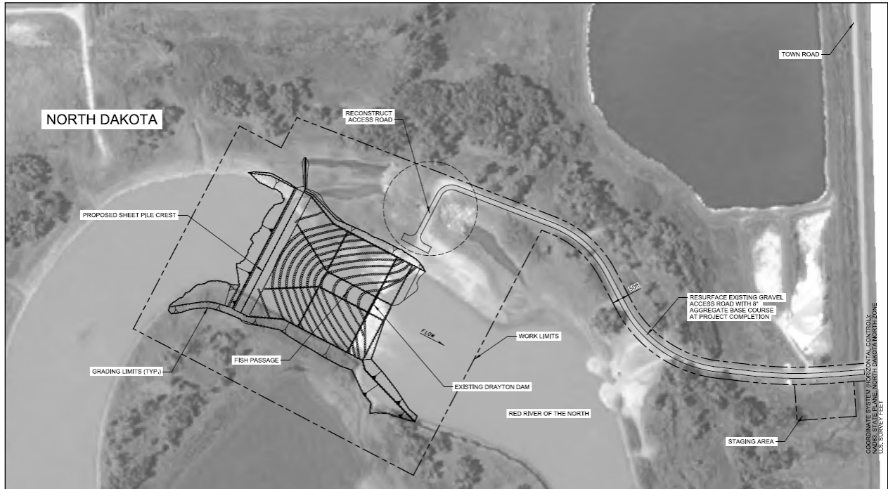
Figure 4. Proposed Drayton Dam fish passage alternative on the Red River of the North. Design and aerial photo are rotated so that the “west” direction is straight up; “north” is directly right.
