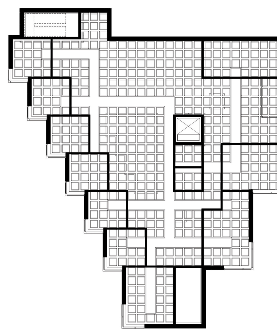
Reflected Ceiling Plan
