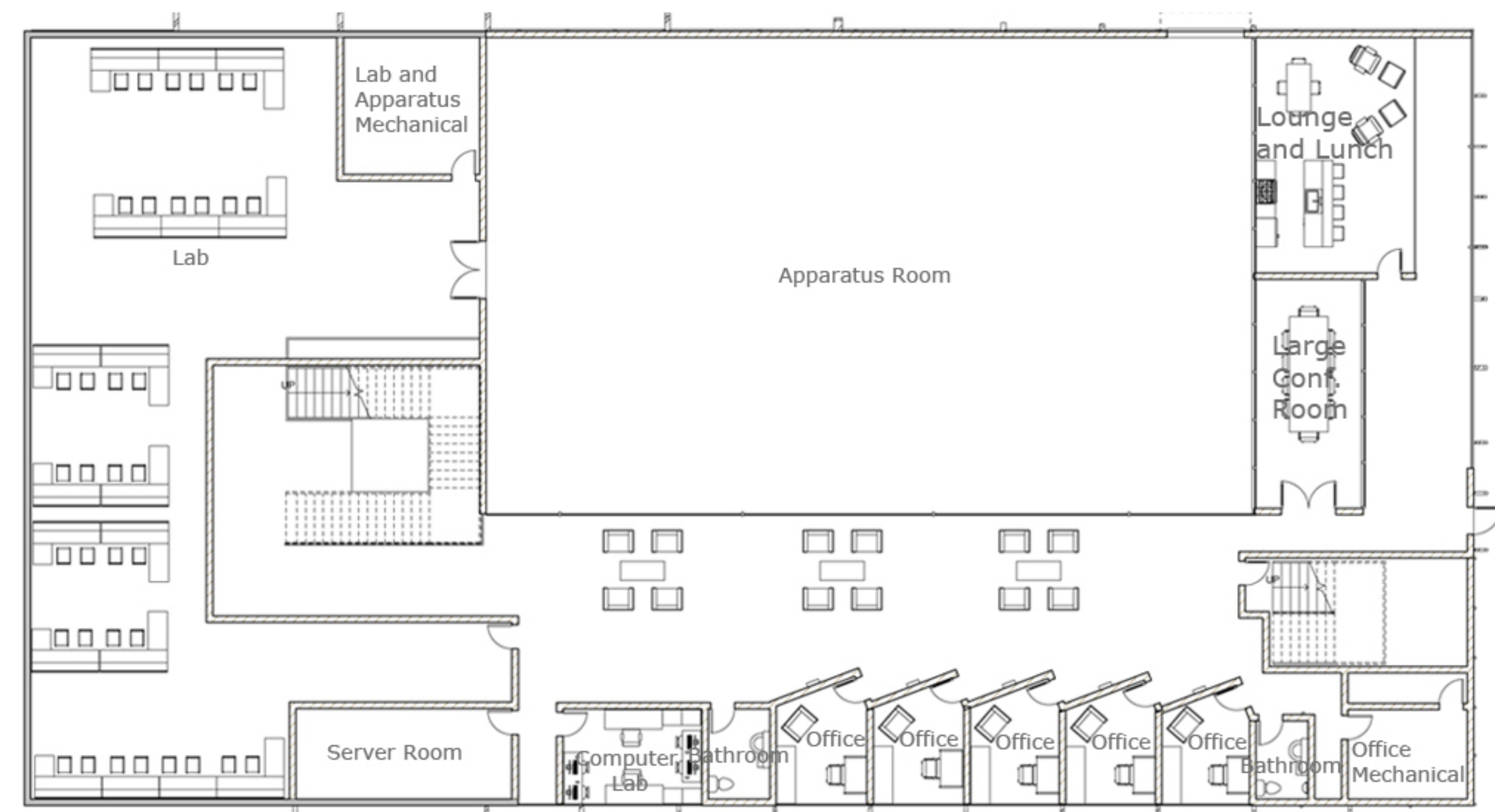
1st Floor
