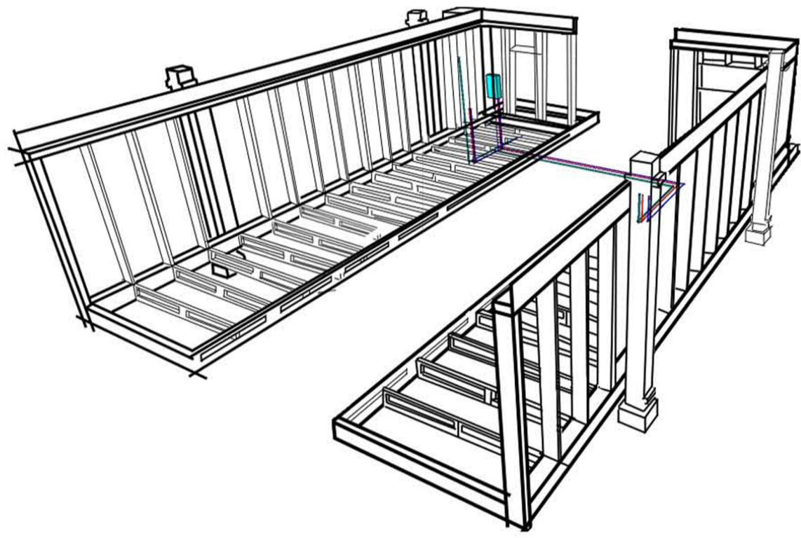
FRAME/UTILITIES
