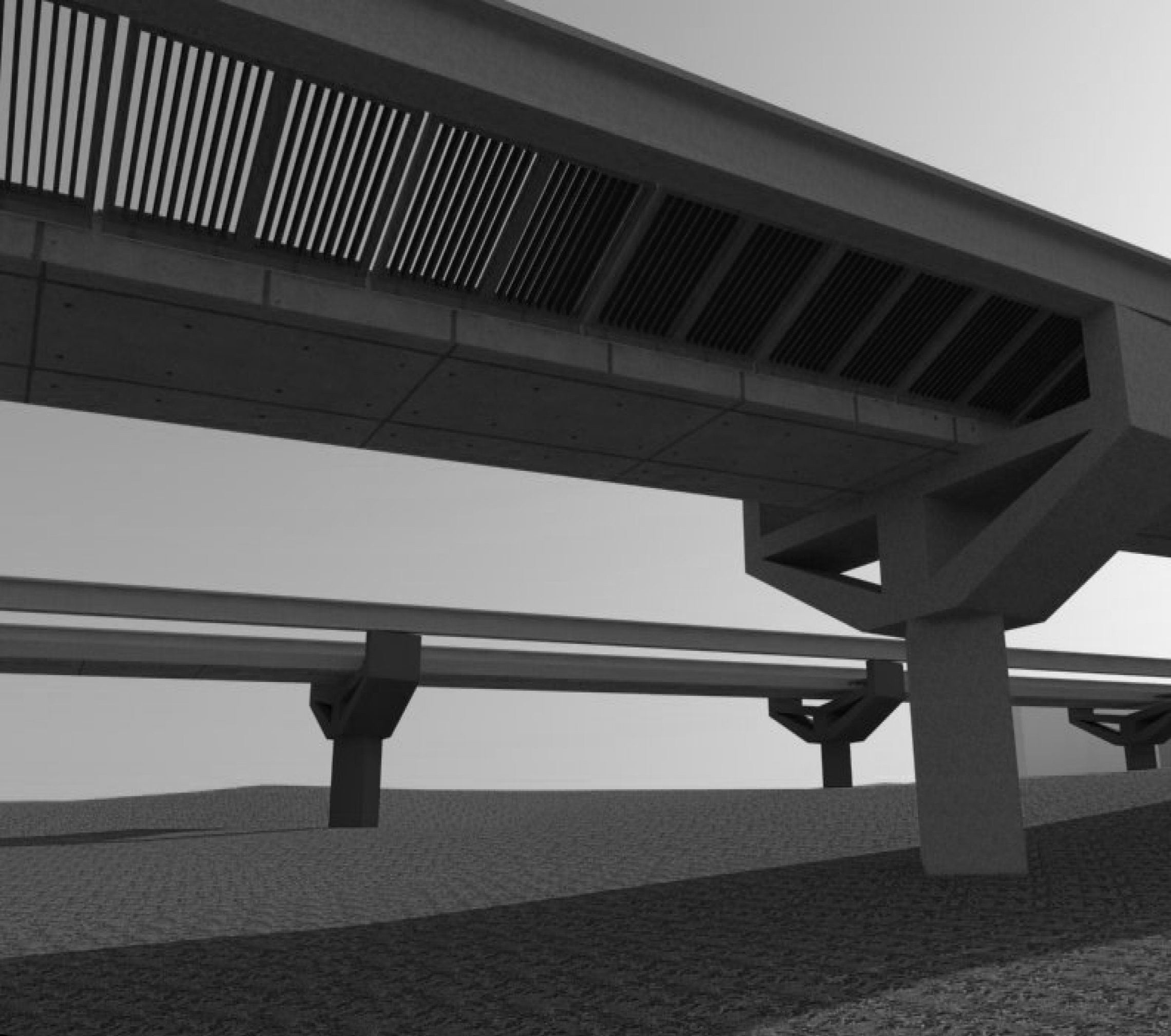
Pre-cast cradle system dropped into place on top of the columns, followed by the concrete slab walkways and permeable grate assemblies.
