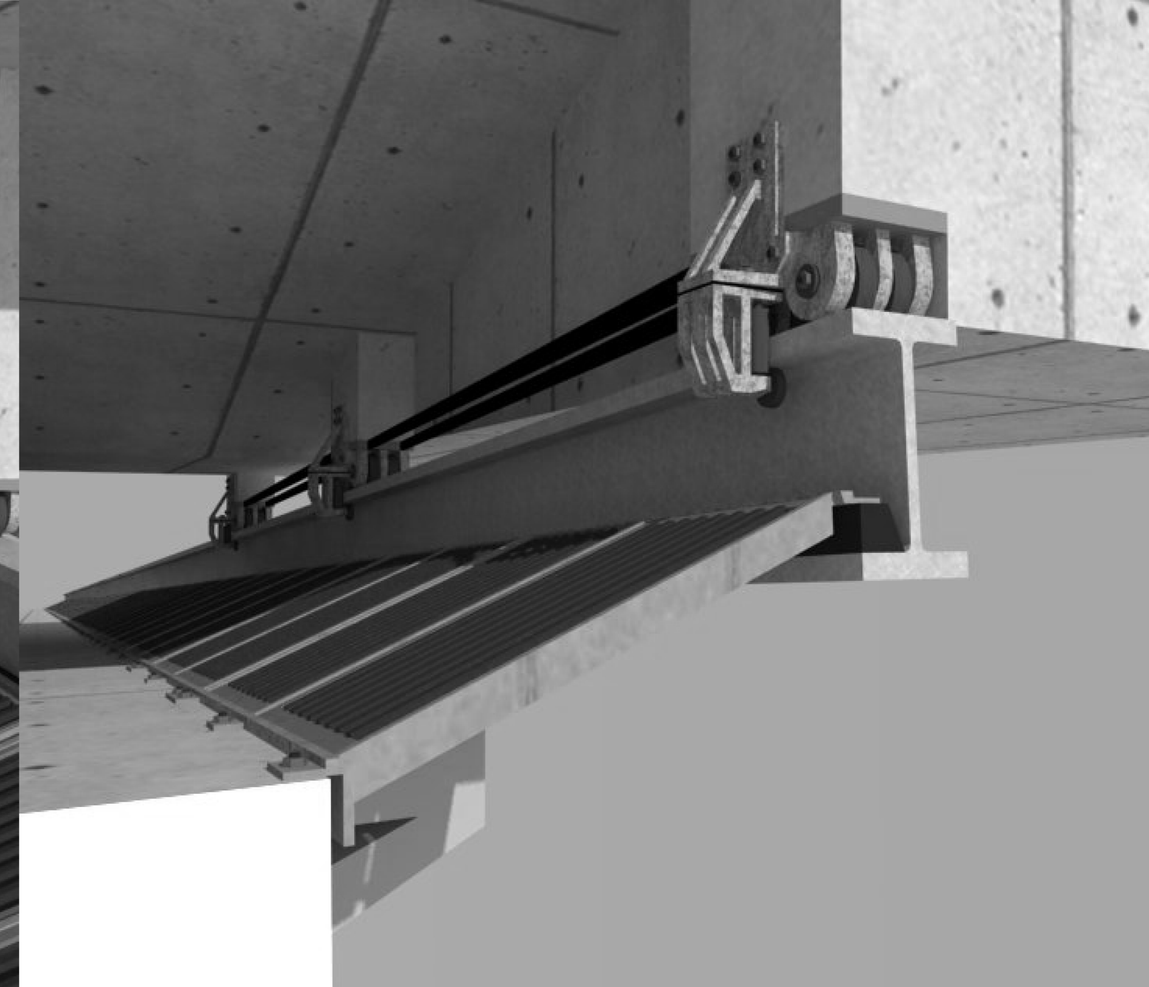
Segmented grate system provides safety while walking on the ramp while still allowing water, light, and air penetration as needed.
