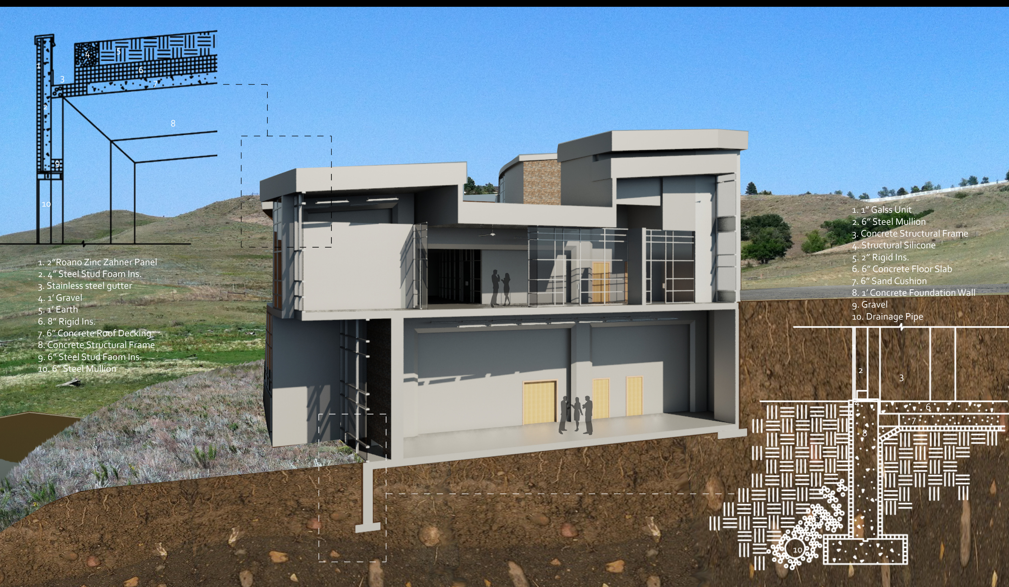
East West Section and Wall Section Details
