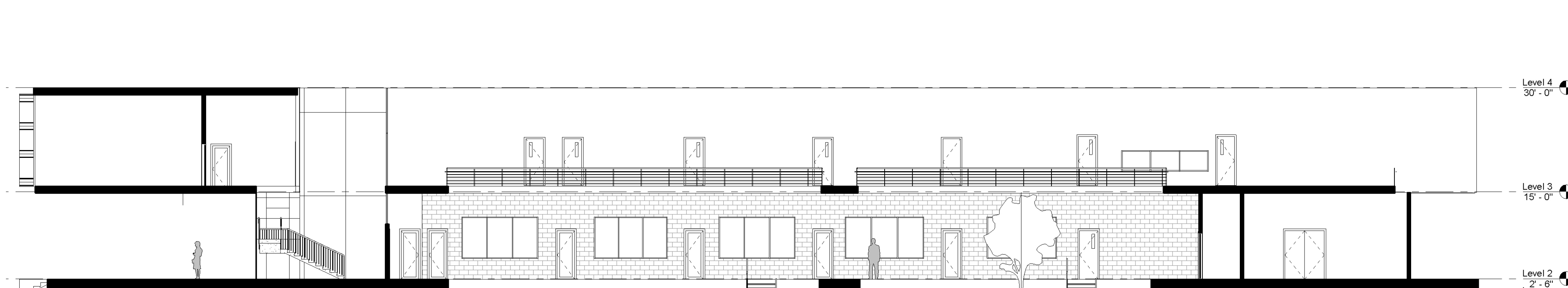
Section
