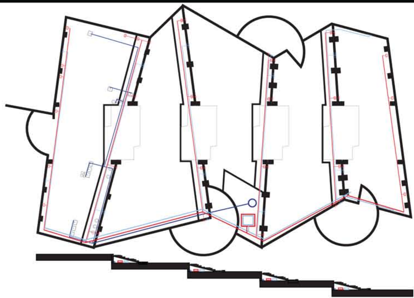
Geothermal heating and cooling ductwork and plumbing run primarily in the spaces provided by the changing levels where floors can overlap, with some branches extending under access floors next to exterior walls. Floor and baseboard grates provide heating or cooling to each space.
