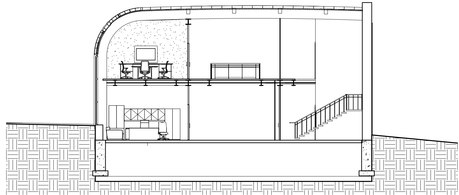
Section 2
