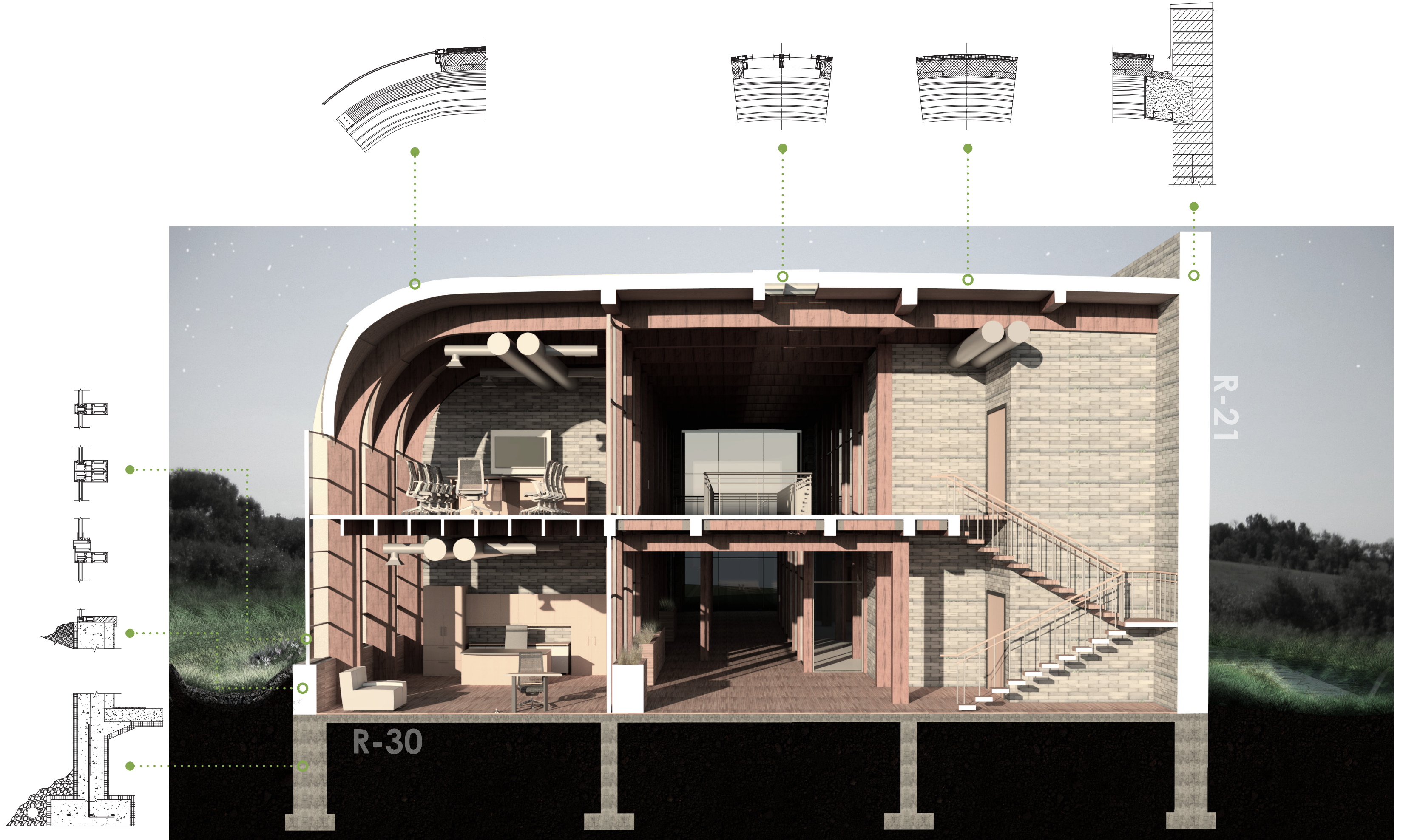
TRANSVERSE SECTION PERSPECTIVE
