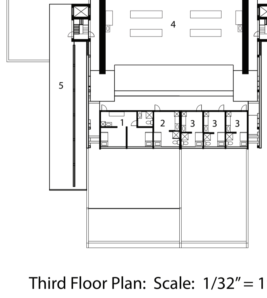
Third Floor Plan: Scale: 1/32" = 1'-0"
