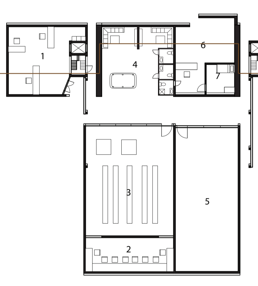
First Floor Plan: Scale: 1/32" = 1'-0"
