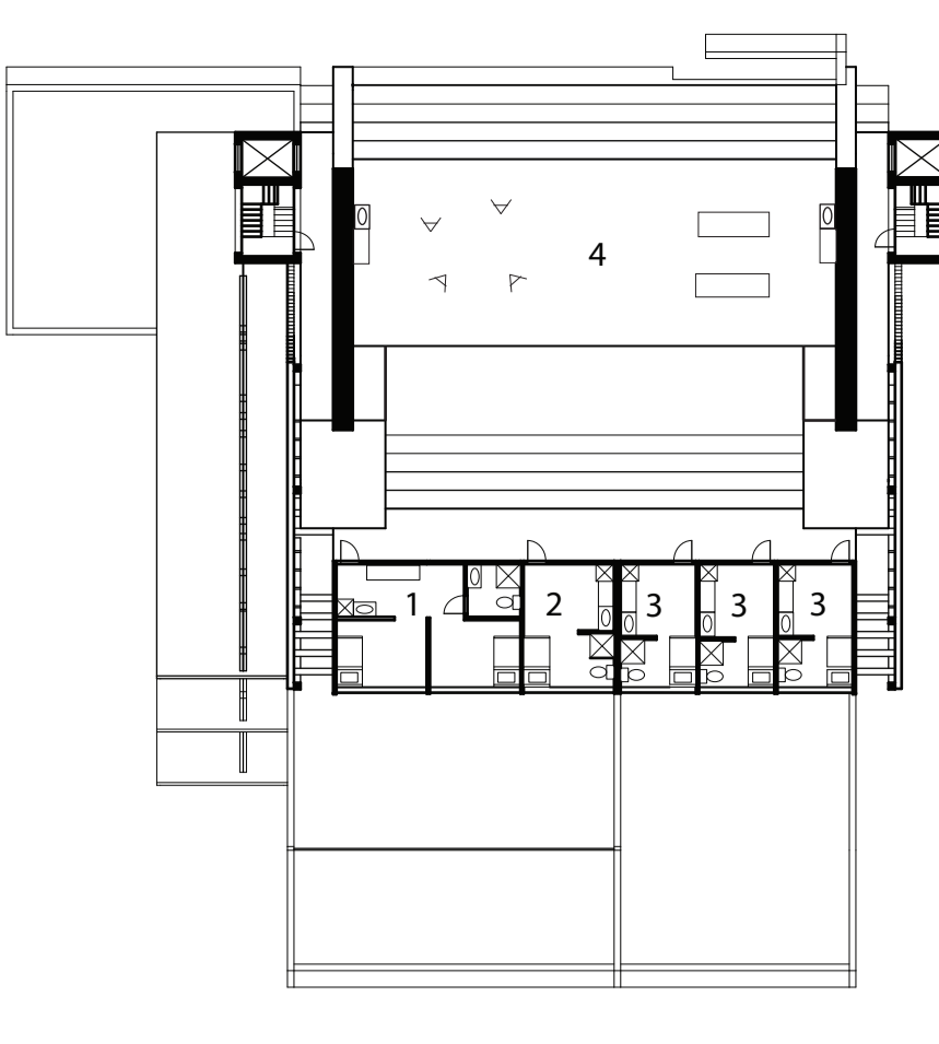
Sixth Floor Plan: Scale: 1/32" = 1'-0"
