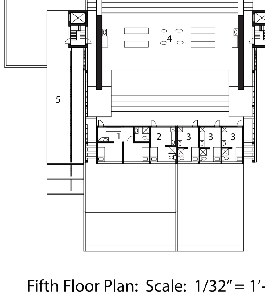
Fifth Floor Plan: Scale: 1/32" = 1'-0"
