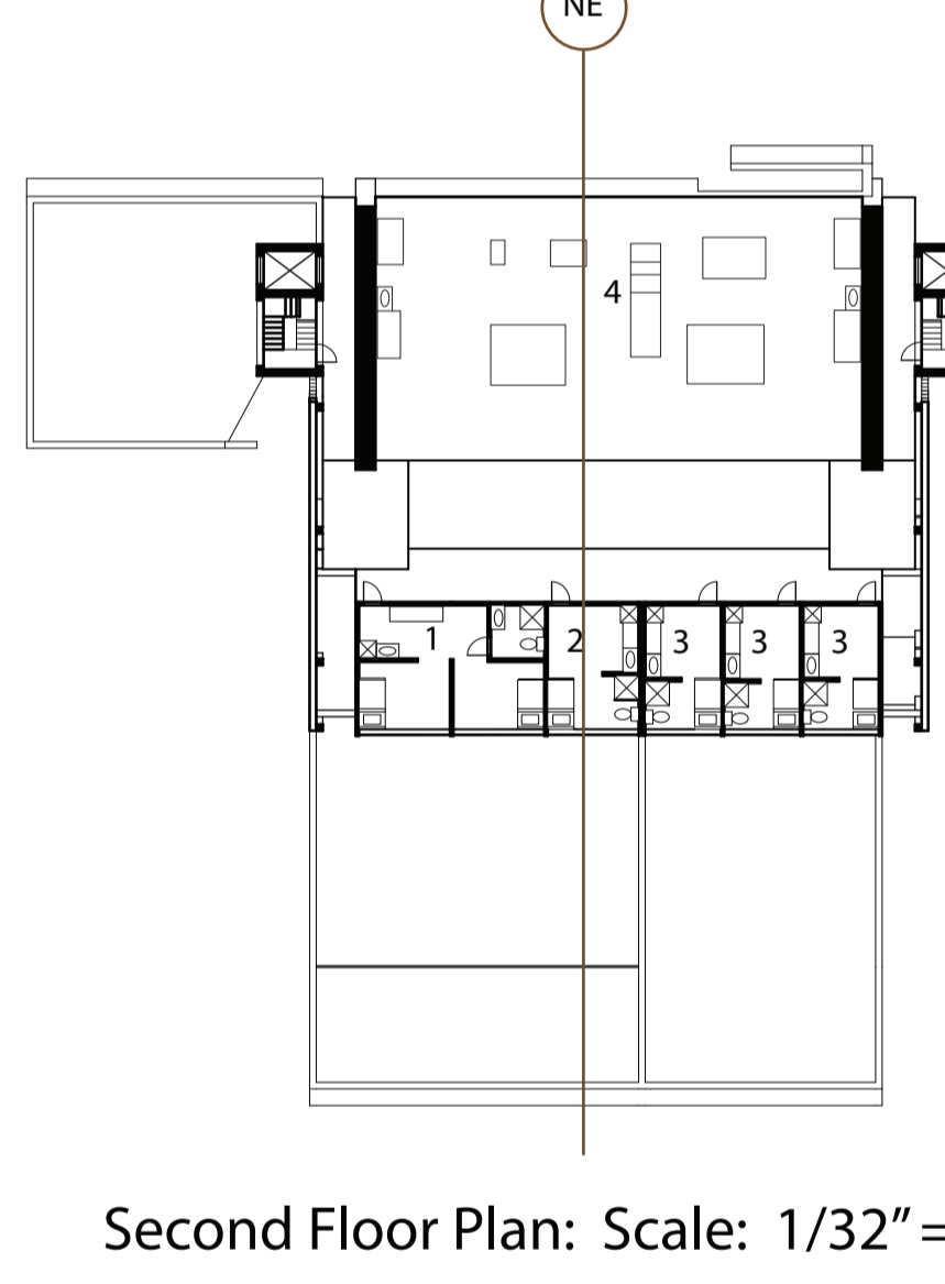
Second Floor Plan: Scale: 1/32" = 1'-0"
