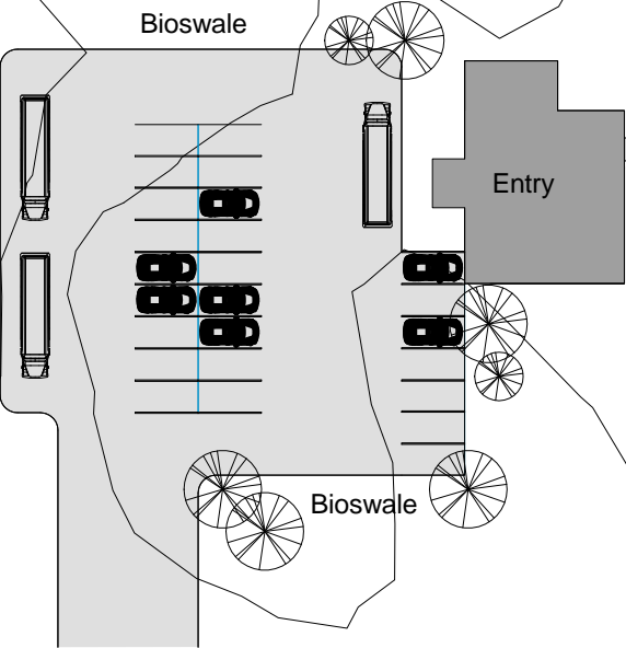
1 Site Plan 1" = 60'-0"
