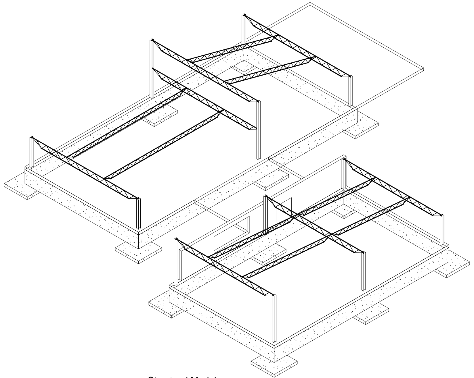
2 Structural Model
