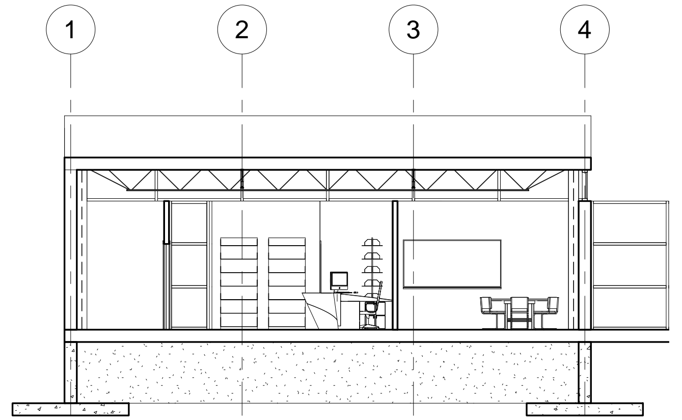
② Lobby 1/8" = 1'-0"
