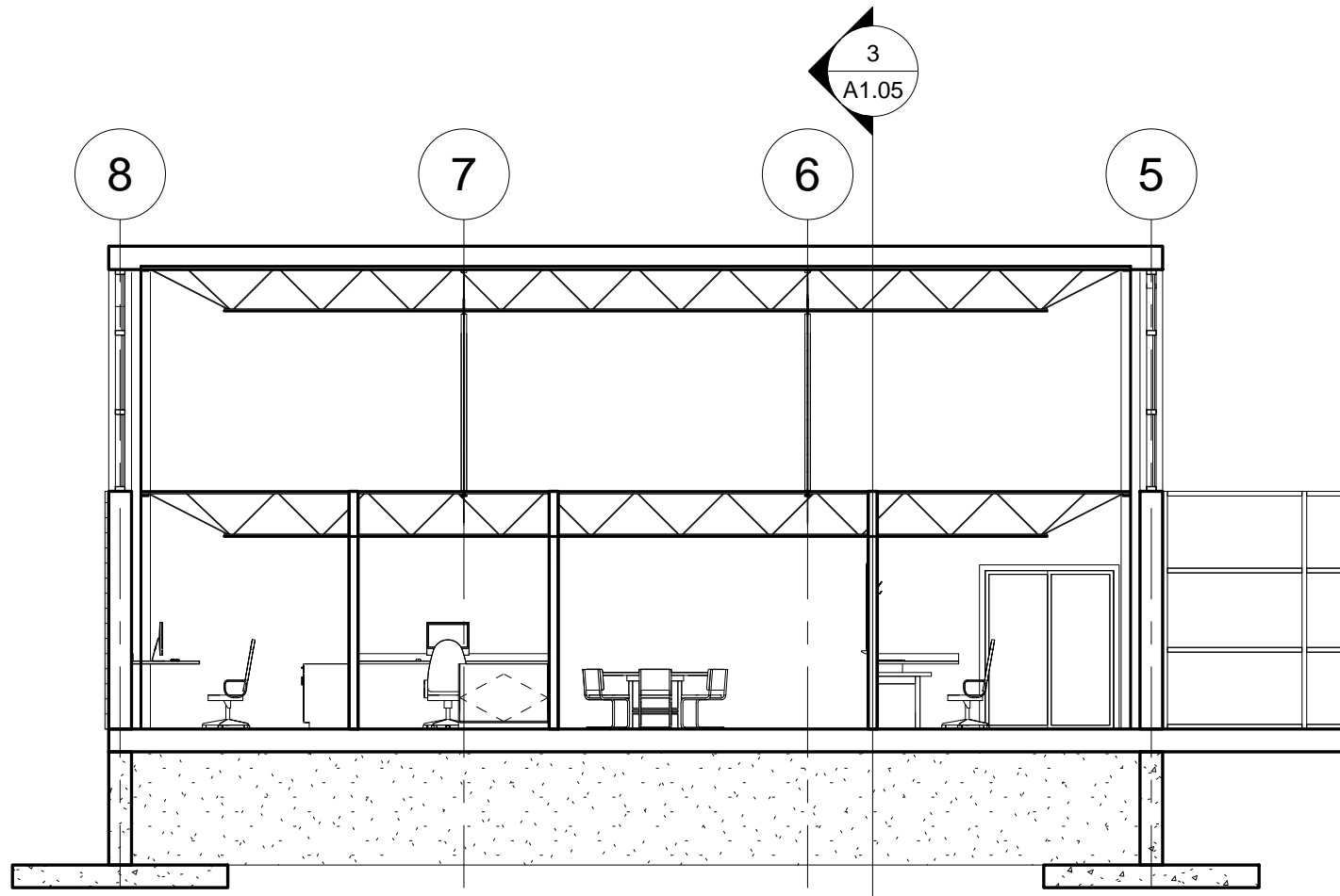
① Office 1/8" = 1'-0"
