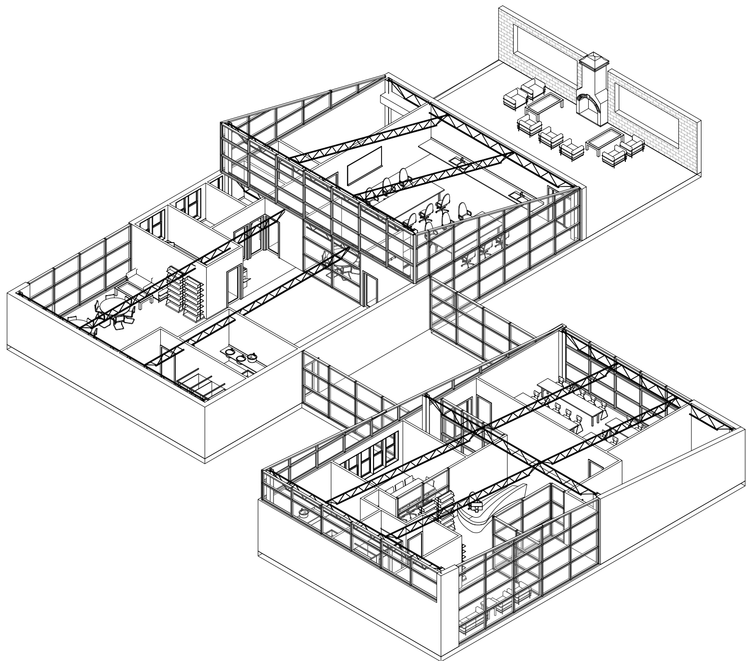
1 Building Model
