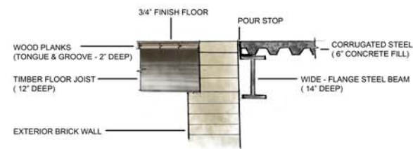
NORTH EXPANSION FLOOR CONNECTIONS
