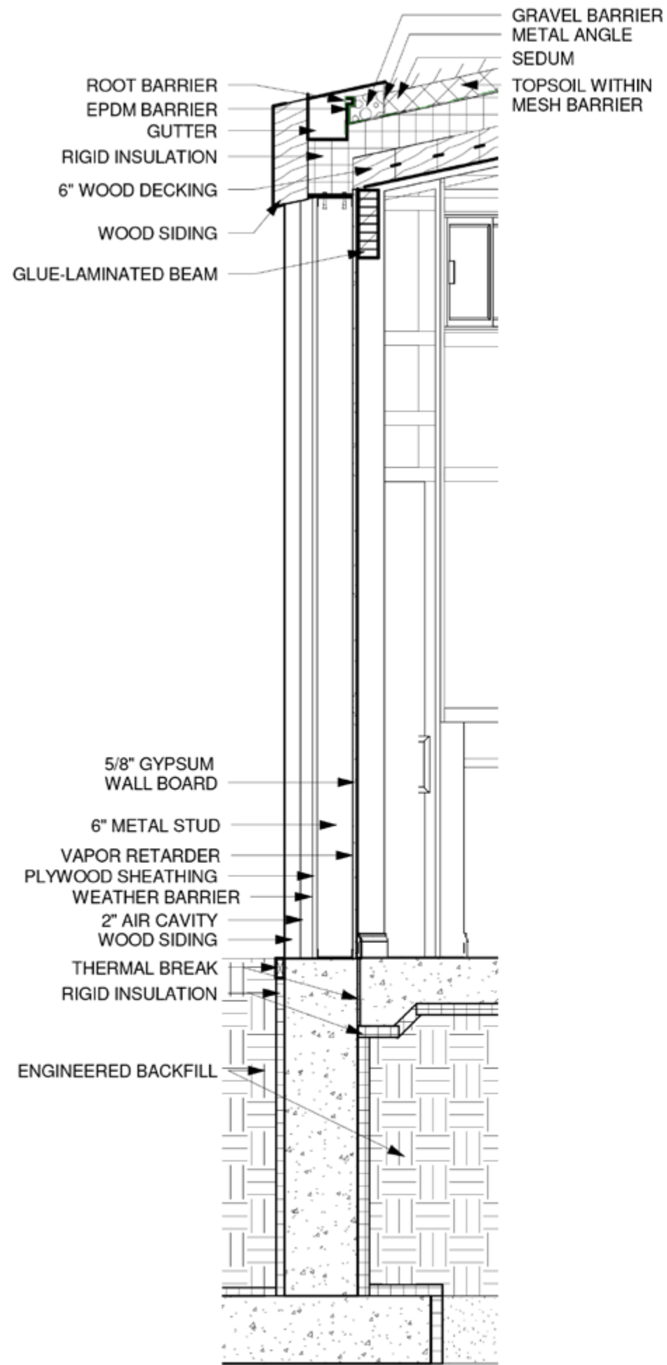
① Gutter at Exterior 1/2" = 1'-0"
