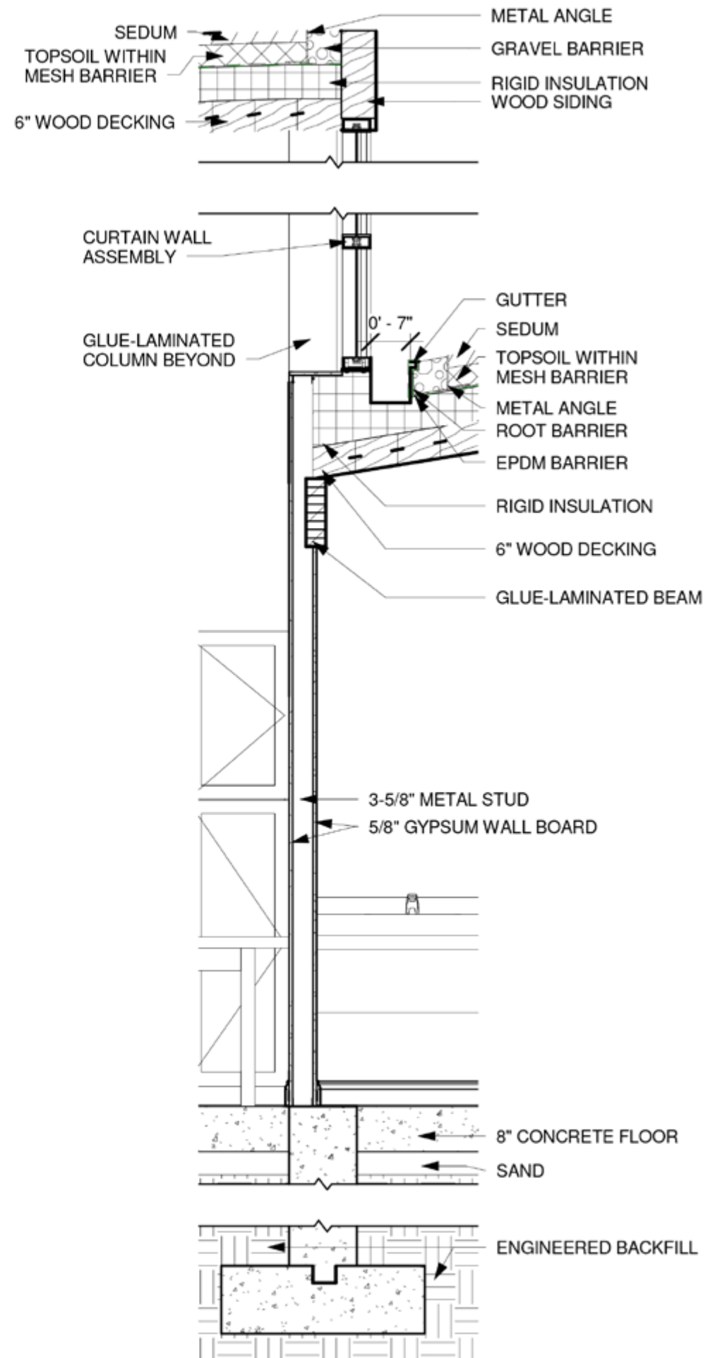
② Gutter at Clerestory 1/2" = 1'-0"
