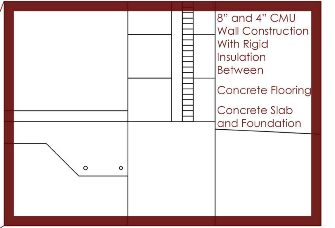
Foundation Detail
