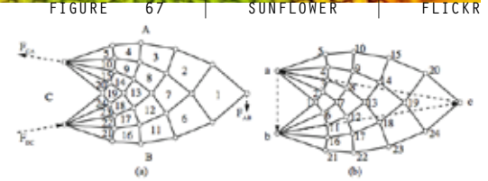
FIG. 5 The solution to the discrete Michell cantilever (Chan 1990; Mazarick et al. 2011) is self-similar of a form diagram, b force diagram. The geometries of the form and force diagrams are the same
