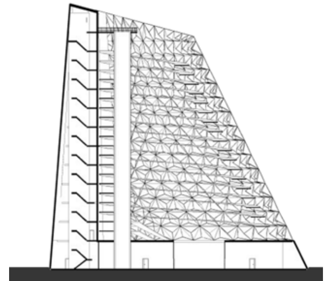
FIGURE 26 | SELF-STANDING SECTION | PLANTAGON
