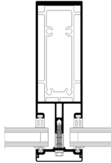
FIGURE 176 | GLAZING SECTION | KRUPNA, TROMETER
