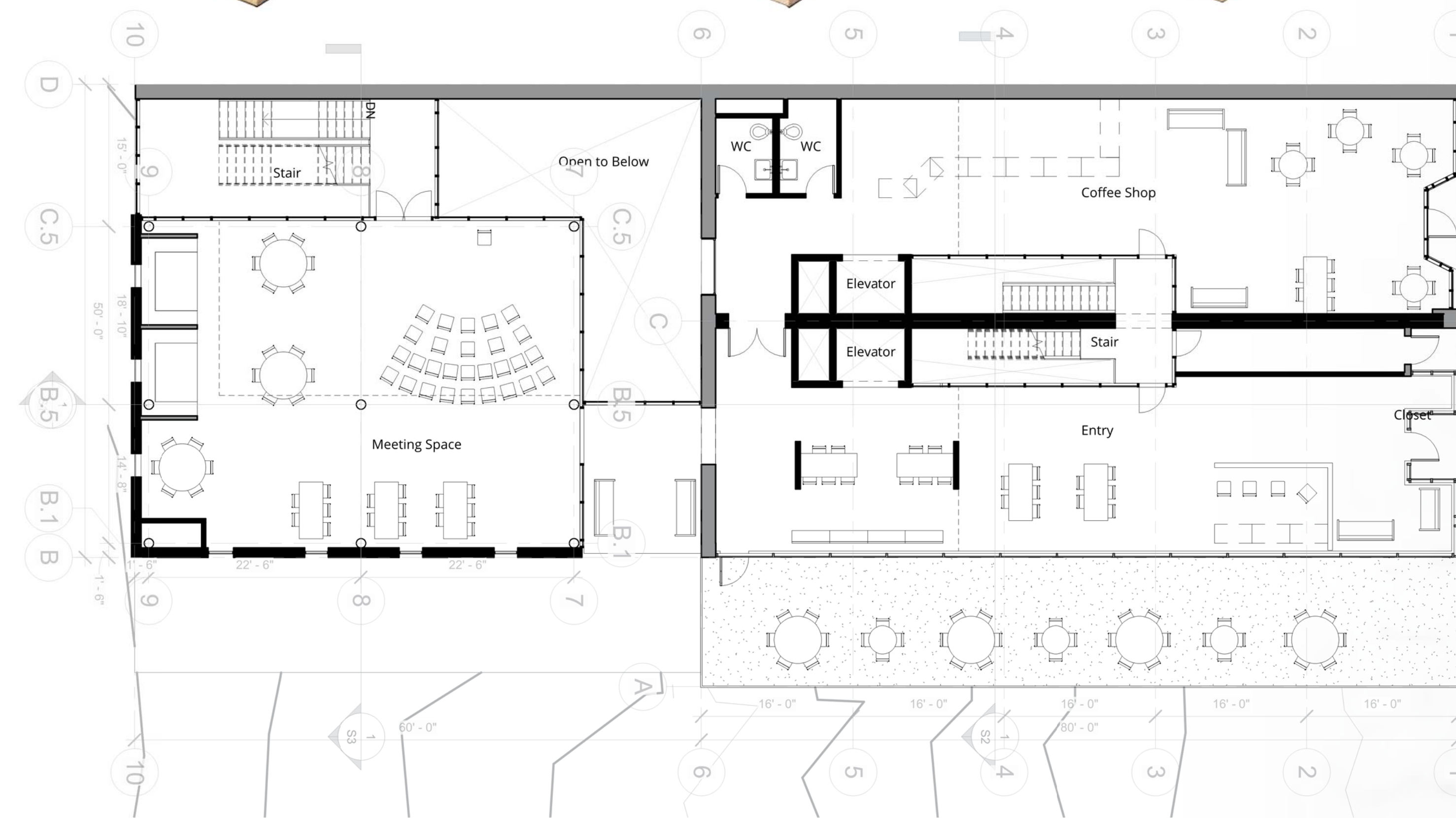
First Level Plan
