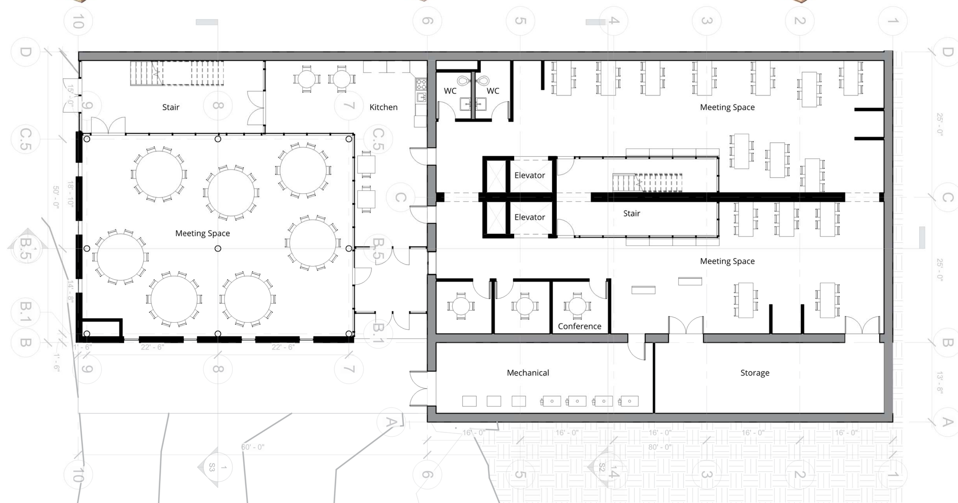
Concourse Plan
