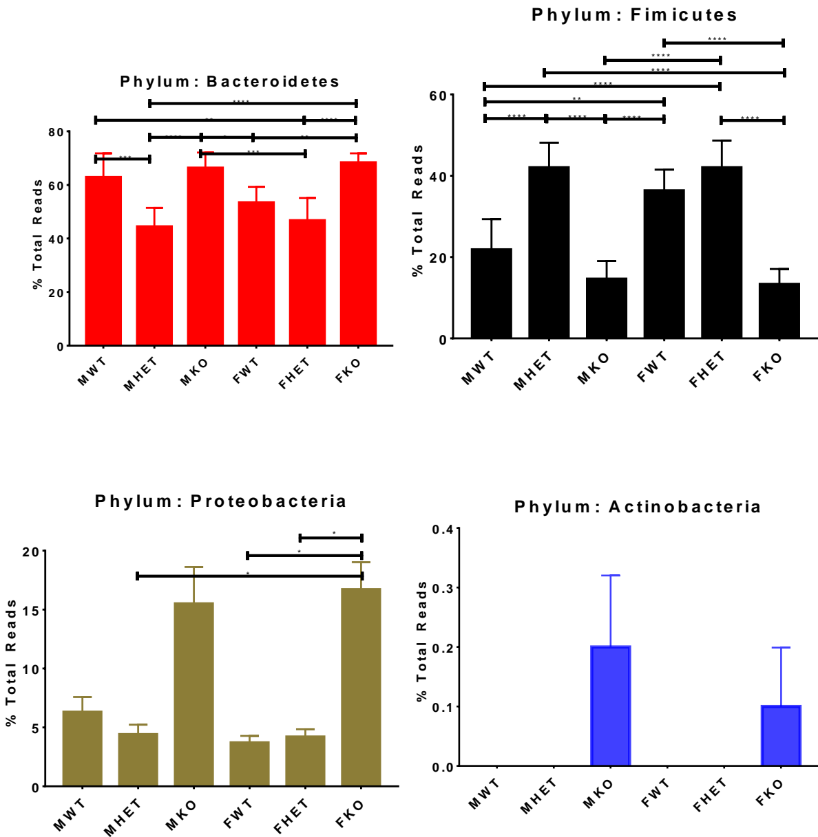
Figure 32. Phylum level statistical differences between VIP strains and sexes. Each bar graph represents an individual phylum and its changes between the mouse strains. The male mice are on the left and the female mice are on the right. The error bars depict calculated SEM values with horizontal lines depicting statistical significance. Stats were run using the Bonferroni test discussed further in 2.2.7.5.
