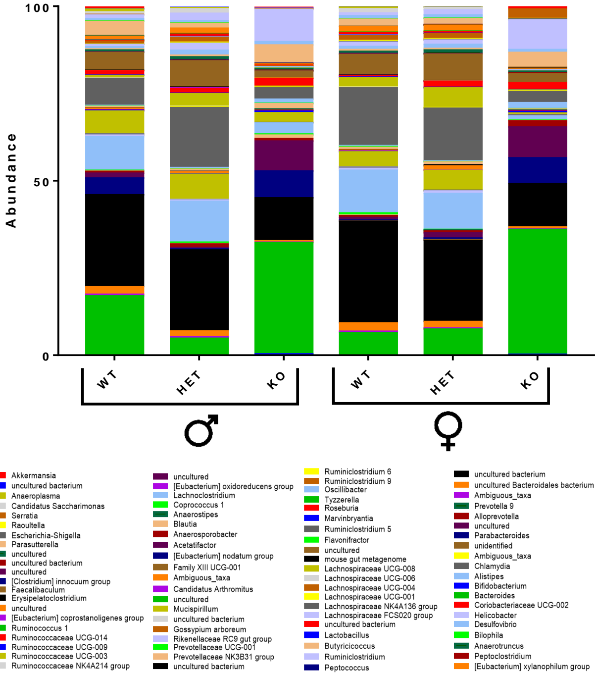
Figure 29. Microbial community changes at the genus level for VIP mouse strains. This stacked bar graph represents the percent abundance of various bacterial genera for each genotype for both sexes. The figure legend depicts an n=8 (7 for male KO) for all strains. The figure legend below the depicts the various color-coded genera. Percent values are available in appendix A.
