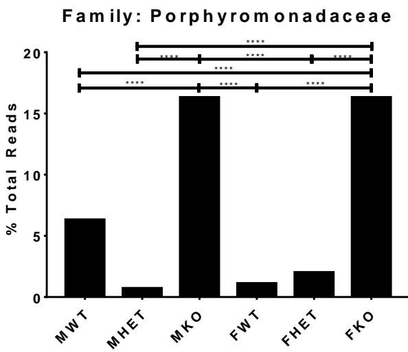
Figure A3. Changes in abundance between individual bacterial families.
