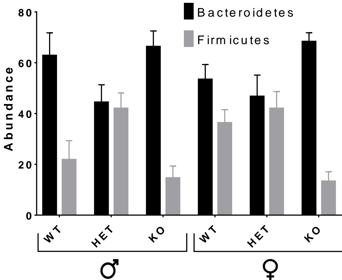
Figure 30. Levels of Bacteroidetes and Firmicutes among the mice strains. A comparative bar graph of the percent abundance of the Bacteroidetes (black) and Firmicutes (gray) phyla found in each mouse strain. The male mice are on the left and the females on the right. The percent abundance of these phyla was averaged across an n = 8 (7 for male VIP KO), across all strains and the error bars indicate SEM values.
