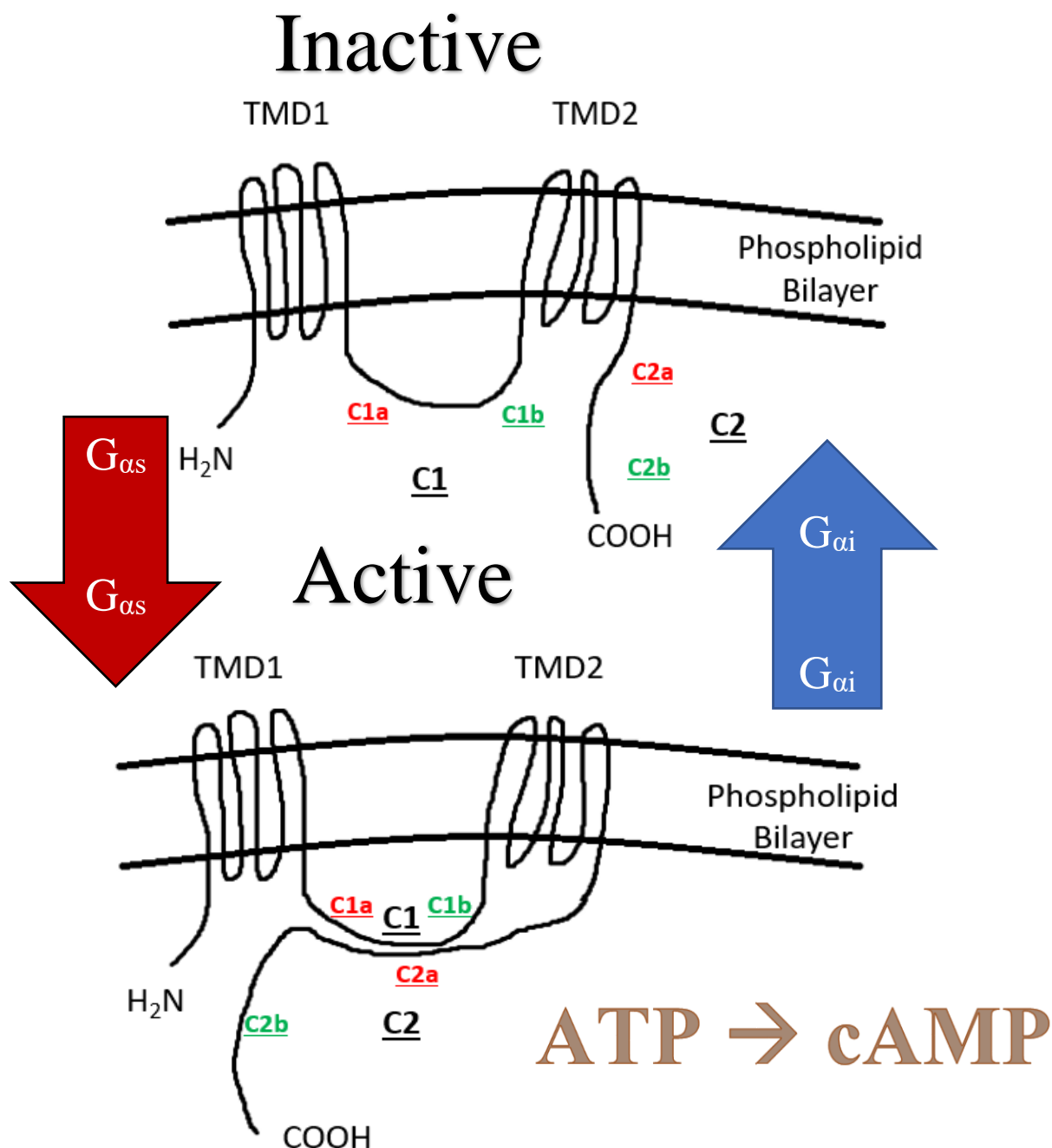
Figure 7. Schematic representation of the enzymatic regulation of AC by G-protein binding. The adenylyl cyclase enzyme contains 12 trans-membrane anchors (TMD1 and TMD2), with a C1 and C2 domain, which needs to become “tethered” together to promote a functional active site for conversion of ATP to cAMP + Pi. Activation by G_{\alpha s} “wraps” the C2a domain over the C1 domain and increases the enzymatic activity of AC. This “wrap” creates a binding site for G_{\alpha i} , which reverses the domain overlap and halts enzymatic activity and subsequent cAMP production.
