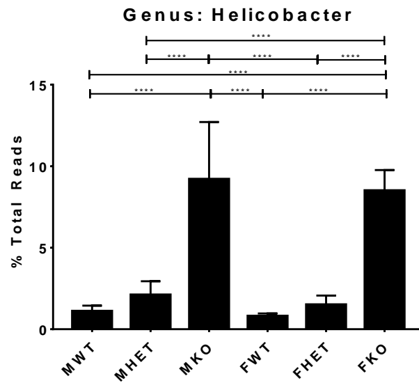
Figure 33. Changes in group 1, Bacteroides, uncultured Porphyromonadaceae and Helicobacter.
