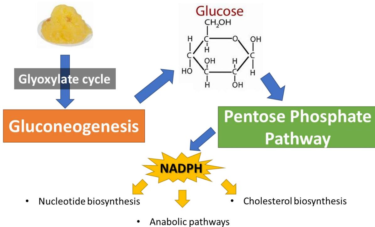
Figure 39. PICRUST results interpretation.
