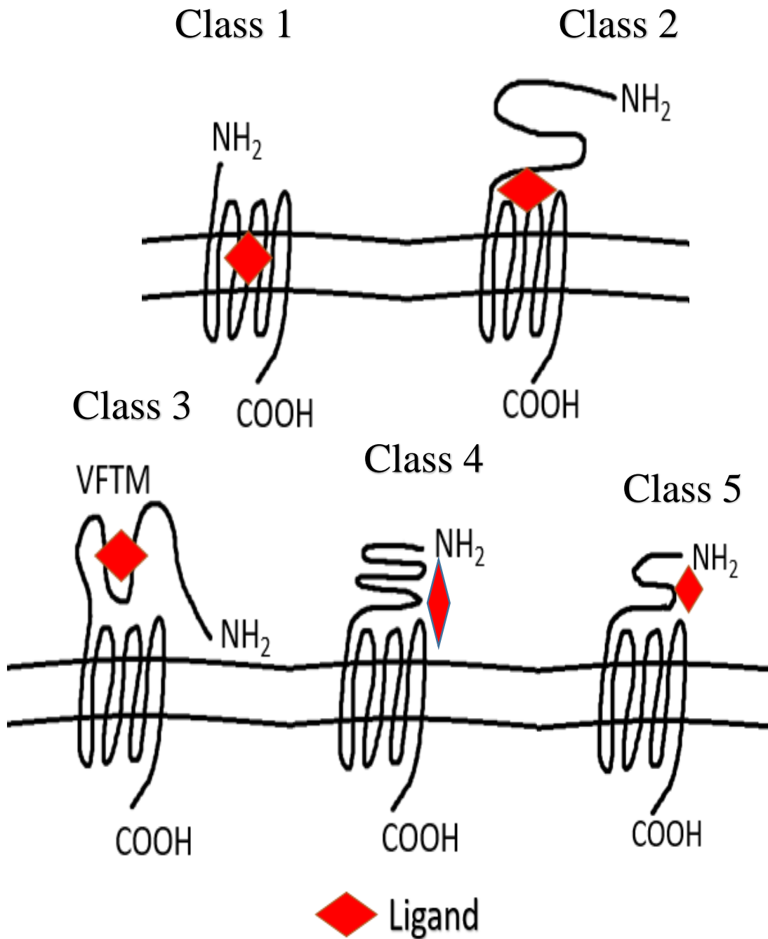
Figure 5. The 5 classes of GPCRs. Schematic representation of all five GPCR classes with ligand binding sites denoted by diamonds. All of these classes share certain defining characteristics. For example, they share a seven-transmembrane region, but the location of ligand binding differs for all five classes as depicted. N-terminus (NH 2 ) and C-terminus (COOH) are indicated for each GPCR class. Venus Fly Trap mechanism (VFTm) is emphasized for class 3 GPCRs.
