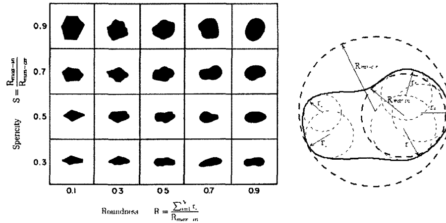
Figure 3-2. Particle shape measurement and Krumbein chart. (Reproduced from G. C. Cho et al., J. Geotechnical. & Geoenvironmental Eng. , 2006, 132, 591)
