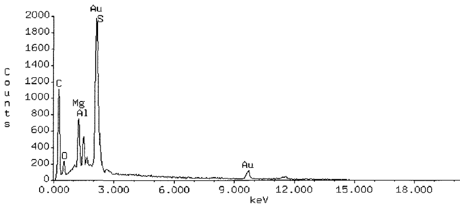
Figure 6-9. EDX spectra of 38% AZ91B Mg alloy-rich primer after exposed in Prohesion chamber for 1328 hours. (b-2) spectrum was obtained from box #1 (on AZ91B pigment particle) and (b-3) spectrum was obtained from box #2 (off pigment particle).
