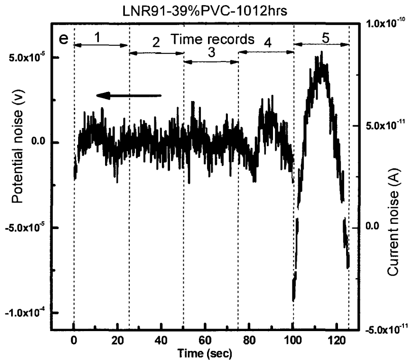
Figure 5-5. ENM data in time domain for the samples coated with 39% PVC LNR91 primer at (a) 157, (b) 356 (c) 663, (d) 856 and (e) 1012 hours exposure. Black lines: potential noise; gray lines: current noise.
