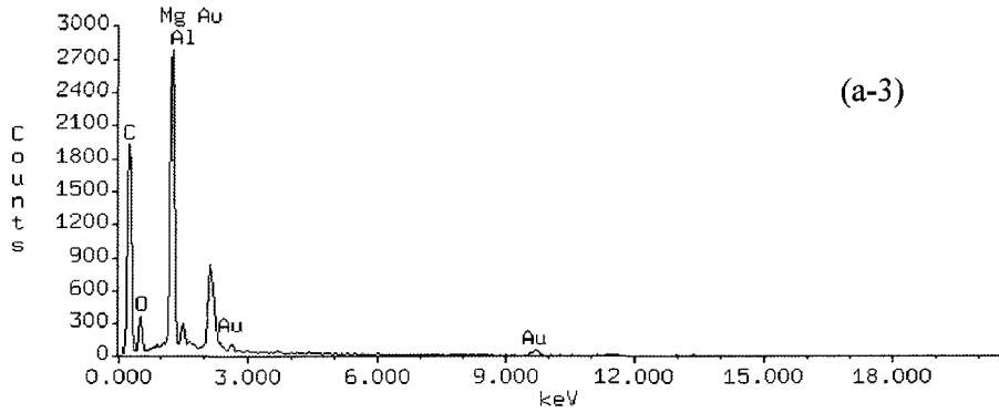
Figure 6-4. SEM image (a-1) and EDX spectra of 34% AM60 Mg alloy-rich primer after exposed in Prohesion chamber for 715 hours. The colored boxes mark the zones for EDX measurement: (a-2) spectrum from box #1(on AM60 pigment particle) and (a-3) spectrum from box #2 (on precipitate).
