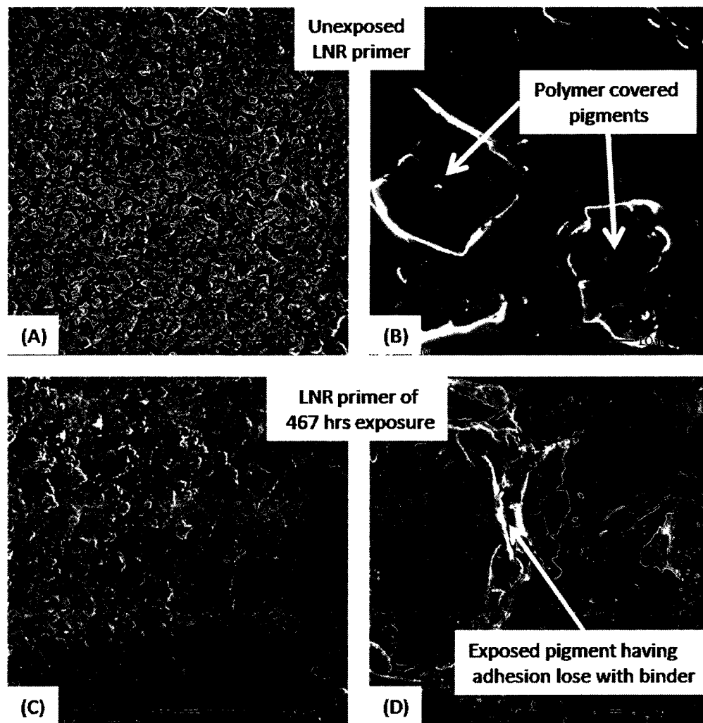
Figure 6-11. SEM surface images of 44% PVC LNR91 pigmented primer: (A) unexposed sample with 25 \times magnification, (B) unexposed sample with 600 \times magnification, (C) sample of 467 hrs exposure with 25 \times magnification and (D) sample of 467 hrs exposure with 600 \times magnifications.
