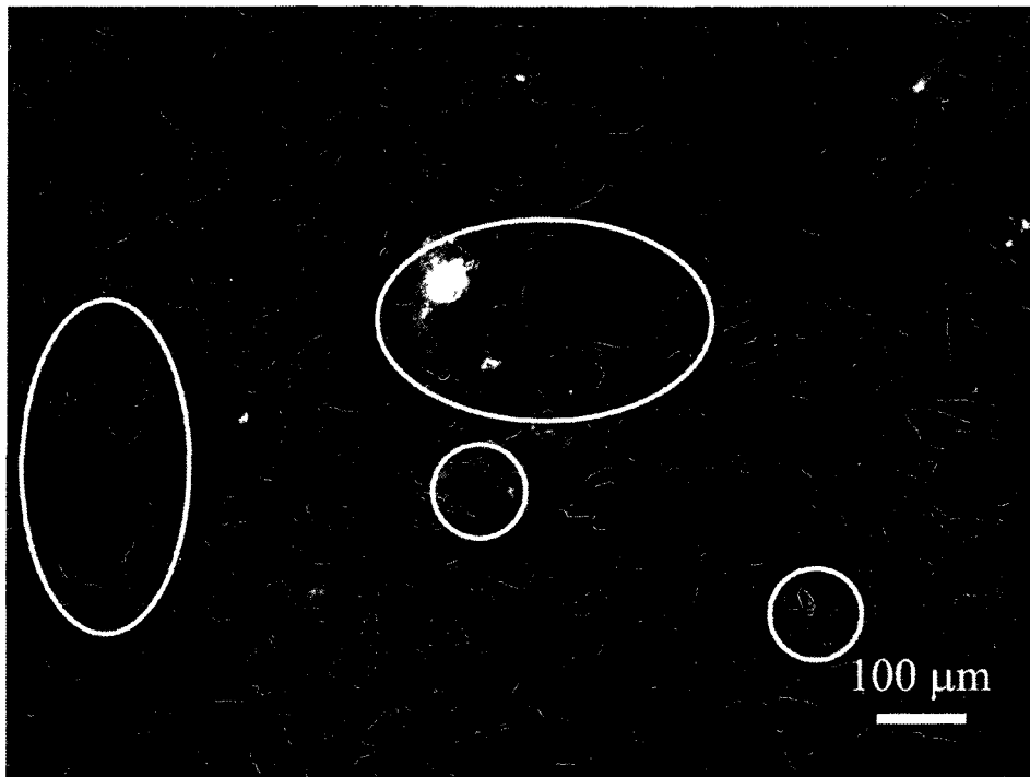
Figure 3-10. Fluorescence image of the presence of coarseness in a 31% PVC AM60 pigmented primer sample: black areas are pigments; gray region is polymer binder; bright spots are voids; the regions marked by white circles show the presence of voids in pigment dense-packing areas (coarseness).
