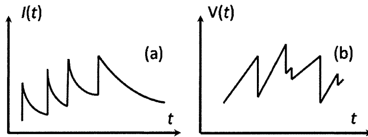
Figure 5-1. Typical time transients of (a) pitting corrosion and (b) uniform corrosion with hydrogen bubble evolution. (Reproduced from F. Huet, Electrochemical Noise Technique , 2006)
