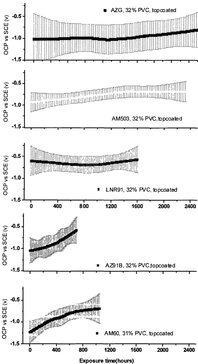
Figure 4-15. OCPs of 32% Mg alloy primer coated panels (with topcoat) as the function of exposure time.
