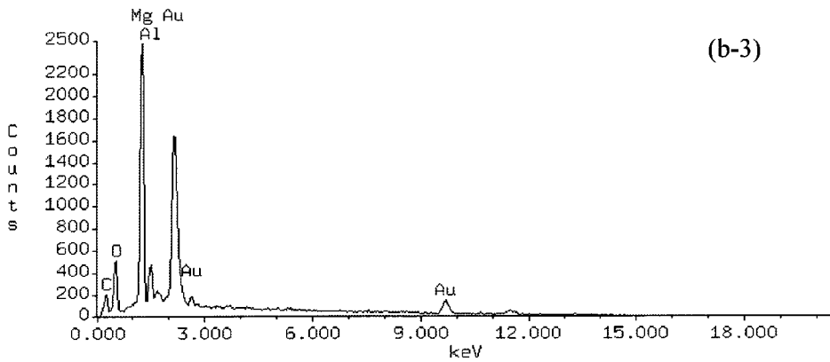
Figure 6-8. EDX spectra of 38% AZ91B Mg alloy-rich primer after exposed in Prohesion chamber for 715 hours. (b-2) spectrum was obtained from box #1 (on AZ91B pigment particle) and (b-3) spectrum was obtained from box #2 (on precipitate).
