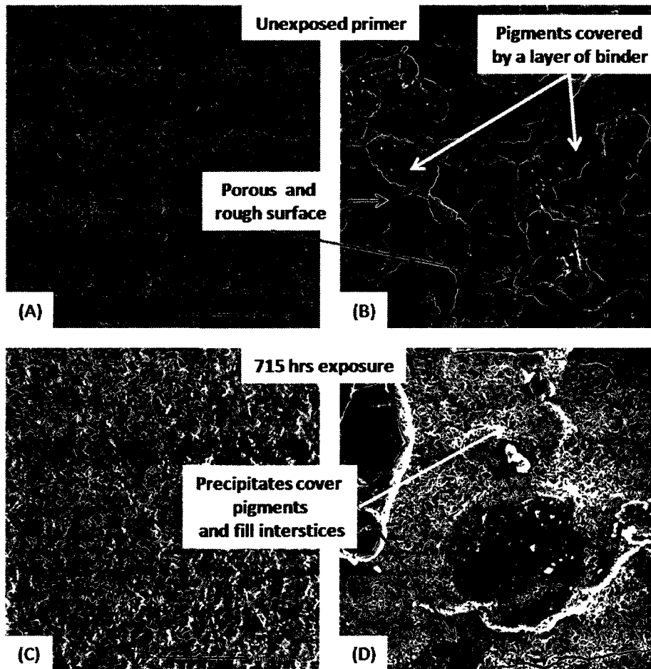
Figure 6-3. SEM surface image of AM60 pigmented primer formulated at 34% PVC: (A) unexposed sample with 25× magnification, (B) unexposed sample with 200× magnification, (C) sample of 715 hours exposure with 25× magnification, (D) sample of 715 hours exposure with 600× magnification.
