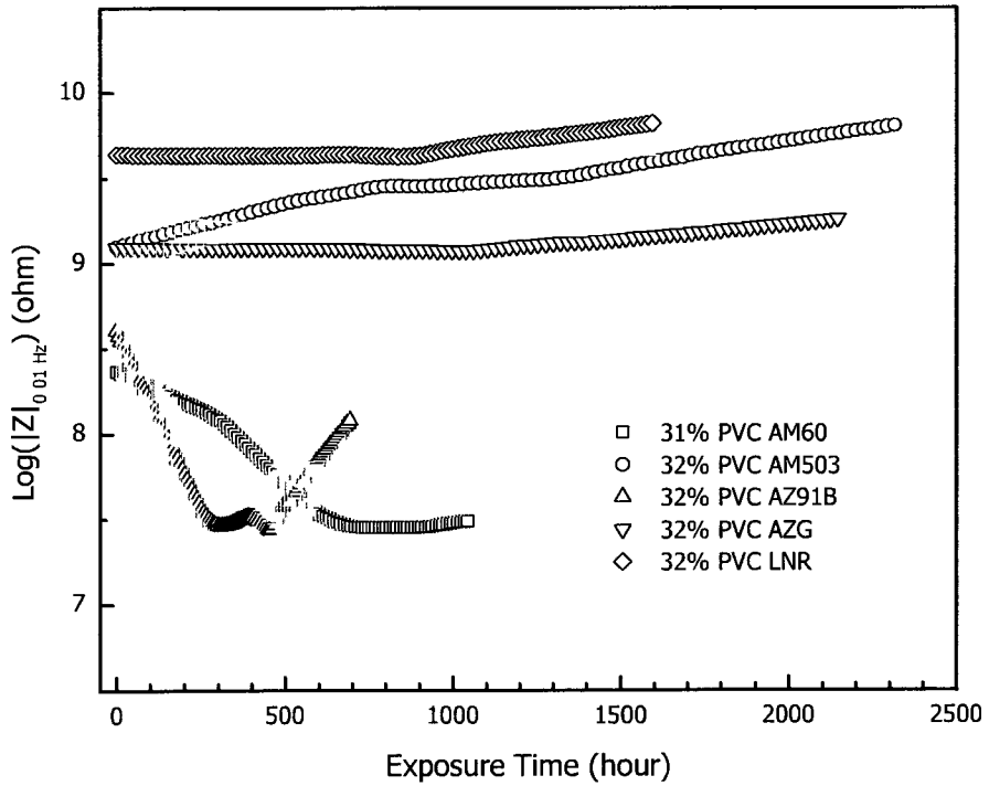
Figure 4-16. |Z|_{0.01\text{Hz}} of Mg alloy primer coated panels (with topcoat) as the function of exposure time.
