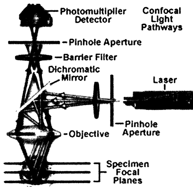
Figure 6-2. Principle of confocal microscopy. (Copied from http://www.olympusfluoview.com/theory/index.html )
