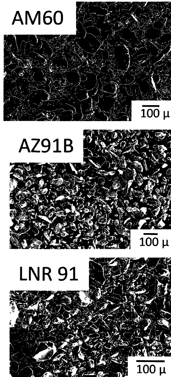
Figure 3-6. Particle shape and morphology of Mg alloy pigments: AM60, AZ91B and LNR91.
