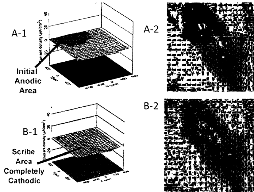
Figure 2-6. 3D SVET plots of current density distribution in the scratched area of Mg-rich primer coated AA2024 T3 sample: (a) immediately after dilute Harrison's solution (DHS) immersion; (b) 30 minutes of DHS immersion. (Copied from G. Bierwagen, et al., Prog. Org. Coat. , 2007 , 59, 172.)
