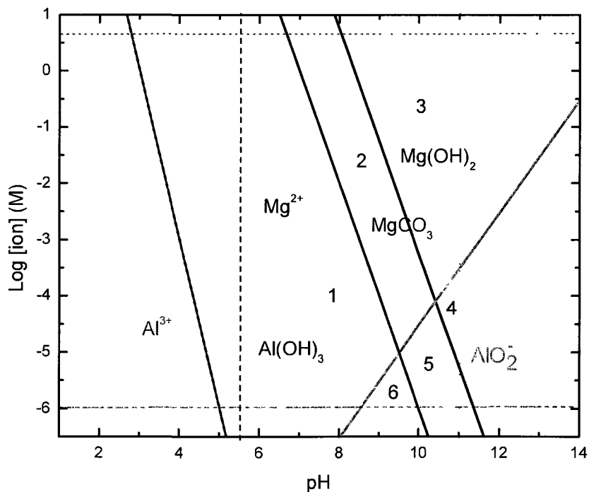
Figure 6-14. Phase diagram of system of Mg alloy oxidation in Prohesion exposure of Mg alloy primer.
