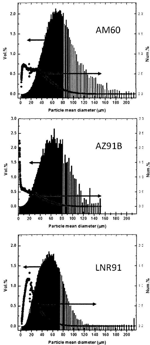
Figure 3-7. Particle size distribution plots of Mg alloy pigments: AM60, AZ91B and LNR91. (Instrument: Accusizer 780 optical particle sizer)
