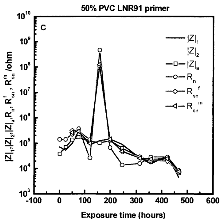
Figure 5-13. Parameters of |Z|_1 , |Z|_2 , |Z|_a , R_n , R_{sn(0.1\text{Hz})}^f and R_{sn(0.1\text{Hz})}^m changes as the function of exposure time for the samples coated with (a)35%, (b) 39% and (c) 50% PVC LNR91 primers.
