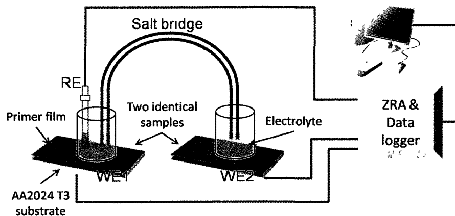
Figure 5-2. Electrochemical cell configuration of three-electrode ENM.
