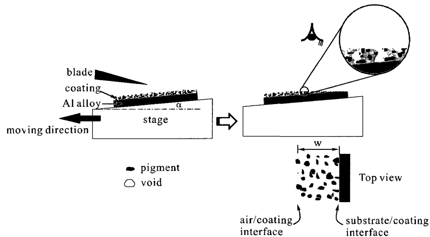
Figure 3-11. Scheme of ultra low angle microtome setup.
