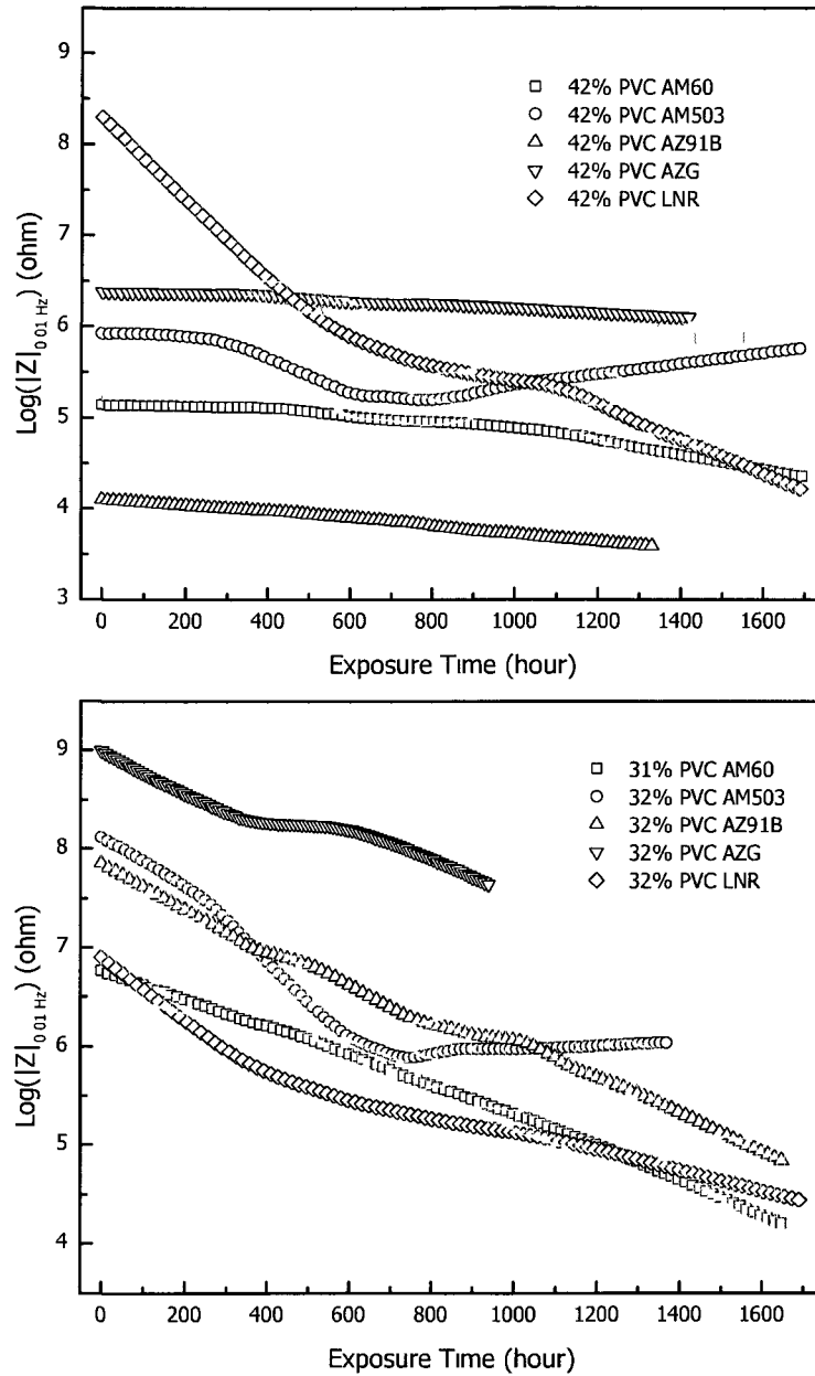
Figure 4-11. \text{Log}|Z|_{0.01\text{Hz}} of AA2024 T3 panels coated with different Mg alloy rich primers (without topcoat) as the function of exposure time.
