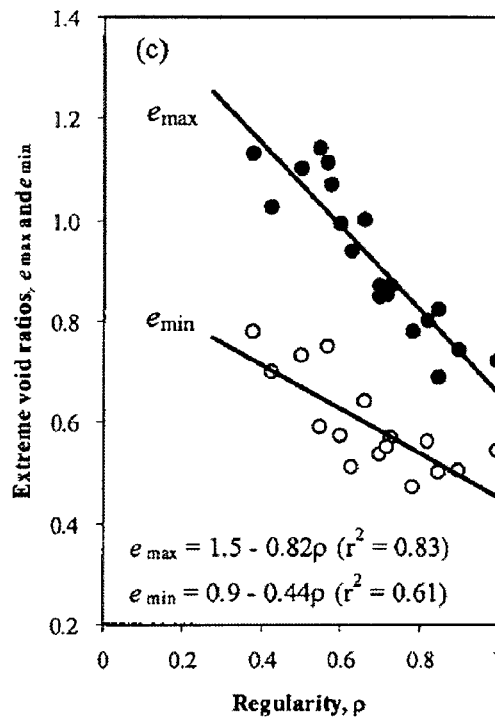
Figure 3-3. Effect of particle shape on extreme void ratios. (Copied from G. C. Cho et al., J. Geotechnical. & Geoenviornmental Eng. , 2006 , 132, 591)
