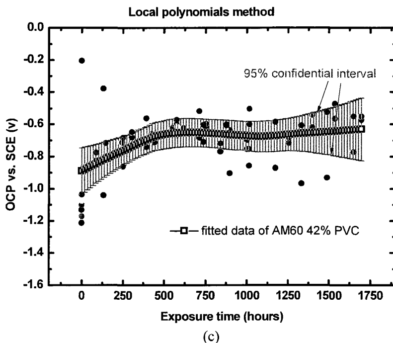
Figure 4-5. Data fitting plots by using (a) kernel estimators ( h=41 ), (b) smooth splines, and (c) local polynomials.
