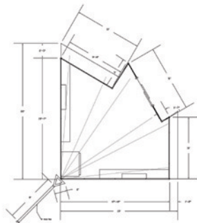
Floorplan Scale 1/4"=1'
