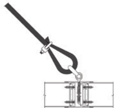
Tensile Connection Detail Scale 6"=1'
