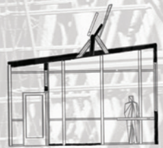
East-West Section 1'=1/4"
