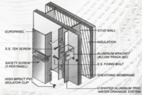
Metal Paneling- Detail
