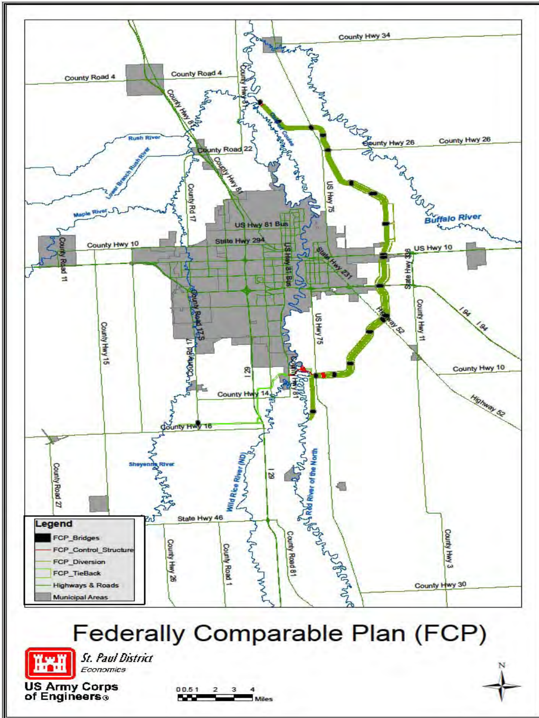
Figure 3 – Federally Comparable Plan (FCP) Diversion Alignment.
