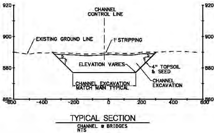
Figure 15 – Typical cross section, bridges, tieback levee, and diversion channel.
