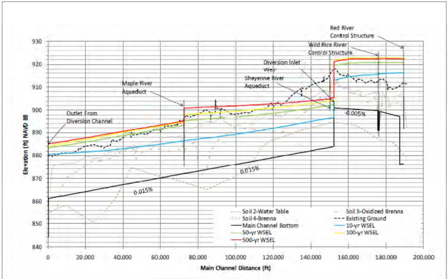
Figure 28 – LPP Channel Profile
