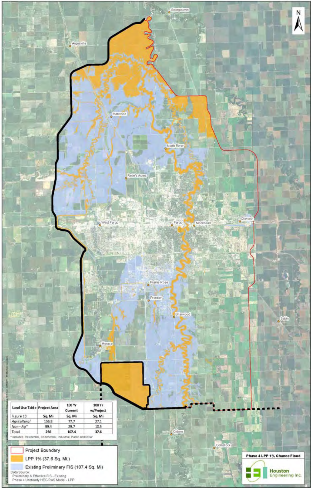
Figure 120 – LPP 1-percent chance event (100-year) floodplain
