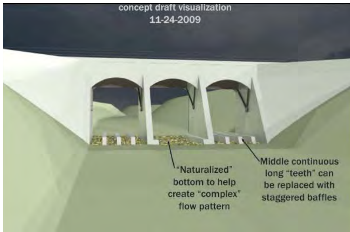
Figure 16 – Conceptual Red River control structure, looking upstream
