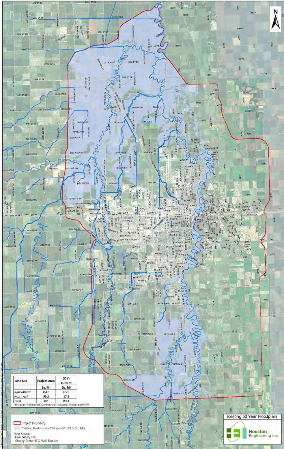
Figure 107– Existing 2-percent chance event (50-year) floodplain.
