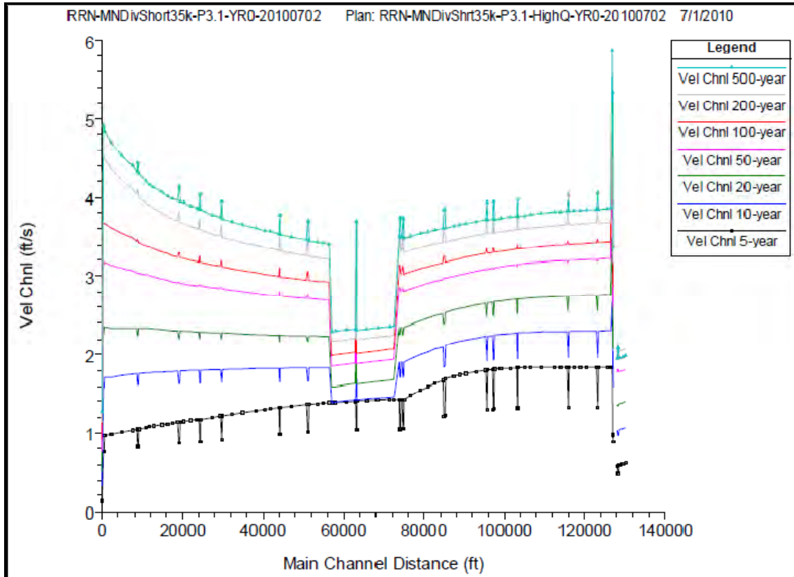
Figure 104 - Average velocities for Red River Diversion channel, FCP alternative, during various discharge events. Velocity estimates begin at the confluence of the diversion channel and the Red River, and extend upstream to the diversion weir. Spikes in velocity plots are due to constrictions at bridge crossings.
