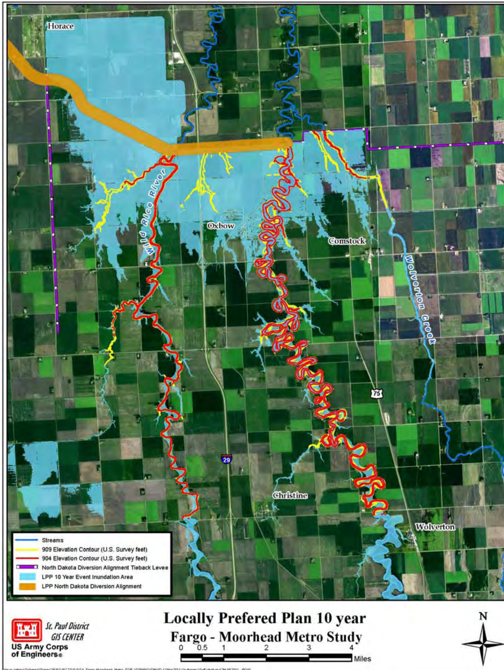
Figure 94 - Area of upstream staging for the LPP during the modeled 10-percent chance event. Map indicates floodplain elevation 909 and 904 ft msl relative to flooded area.
