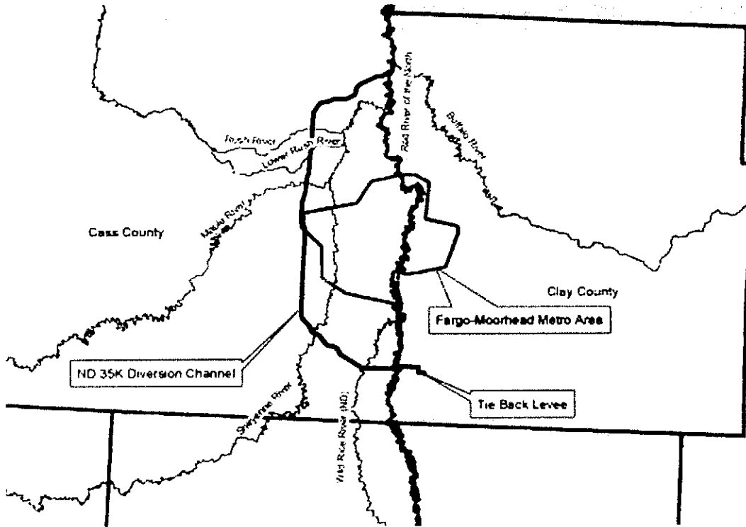
Figure 4. Proposed ND 35K Diversion Channel Alternative
