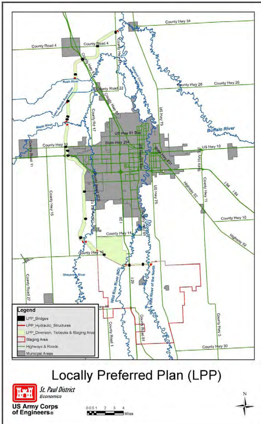
Figure 38 - LPP Diversion Alignment & Features
