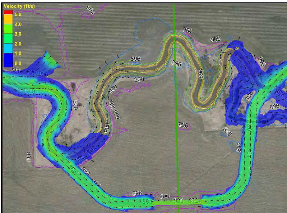
Figure 103 - Average velocities for the Maple Aqueduct under the LPP for a discharge equal to a 2-year event.
