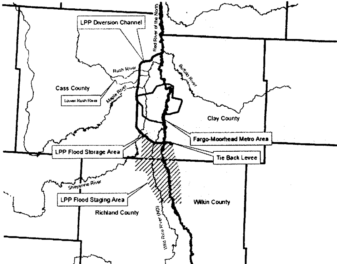
Figure 2. Proposed LPP Diversion Channel Alternative
