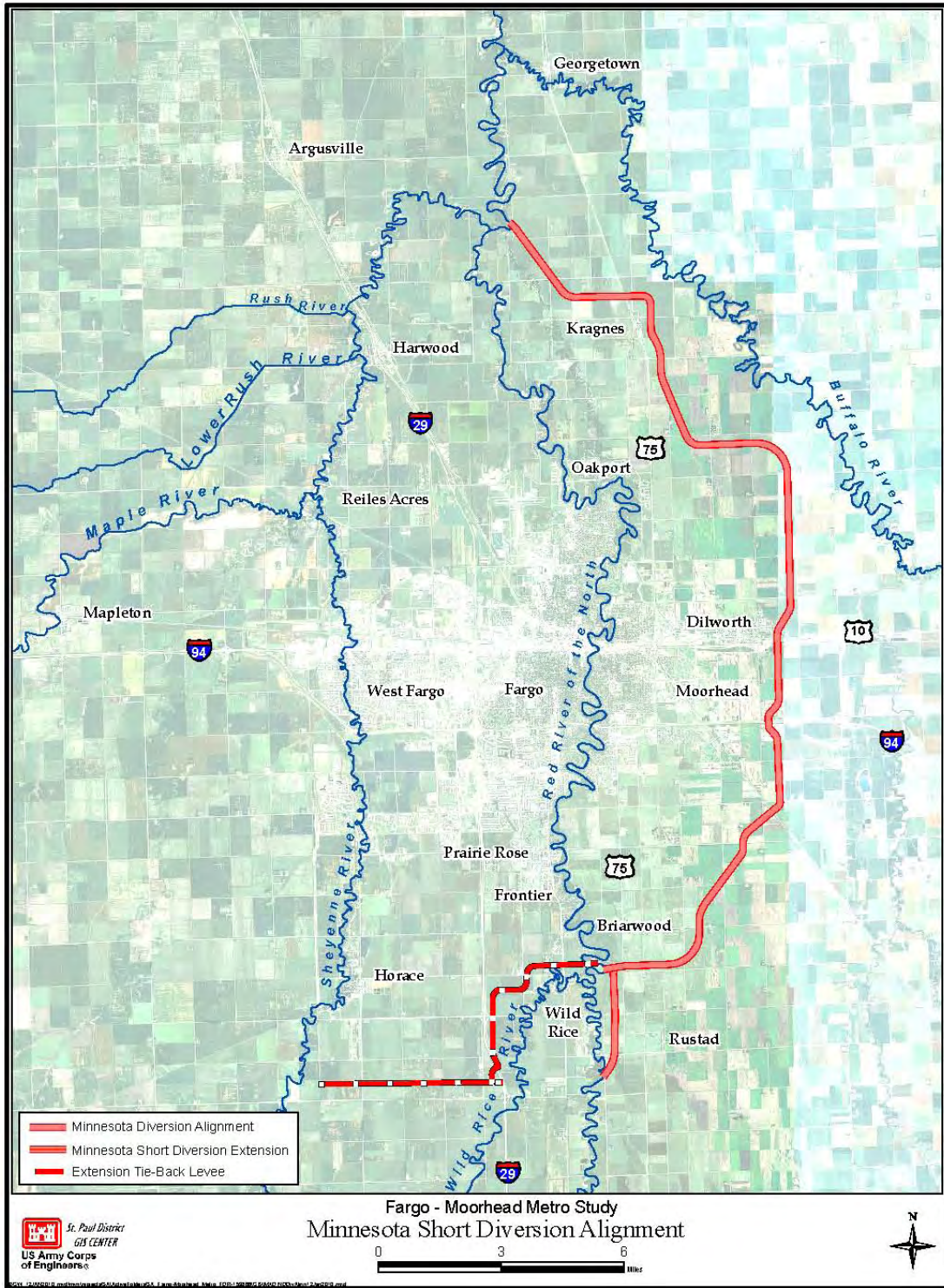
Figure 14 - Minnesota Short Diversion alignment
