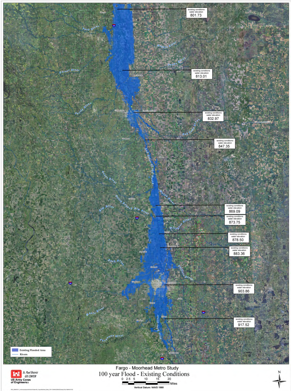
Figure 43 – 1-Percent Chance Flood – Existing Conditions
