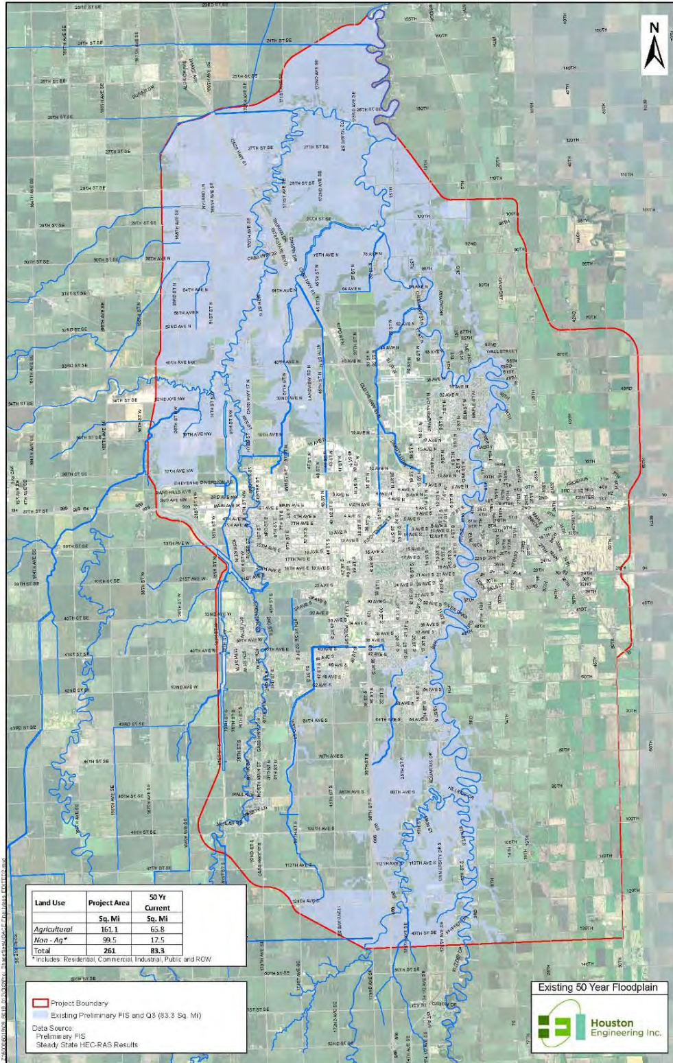
Figure 10 – Existing 50-year floodplain (2-percent chance)
