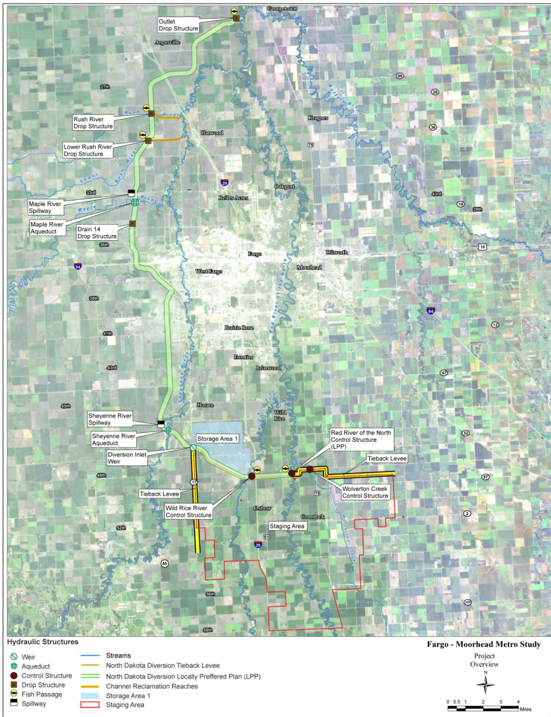
Figure 4 – LPP Diversion Alignment and Features
