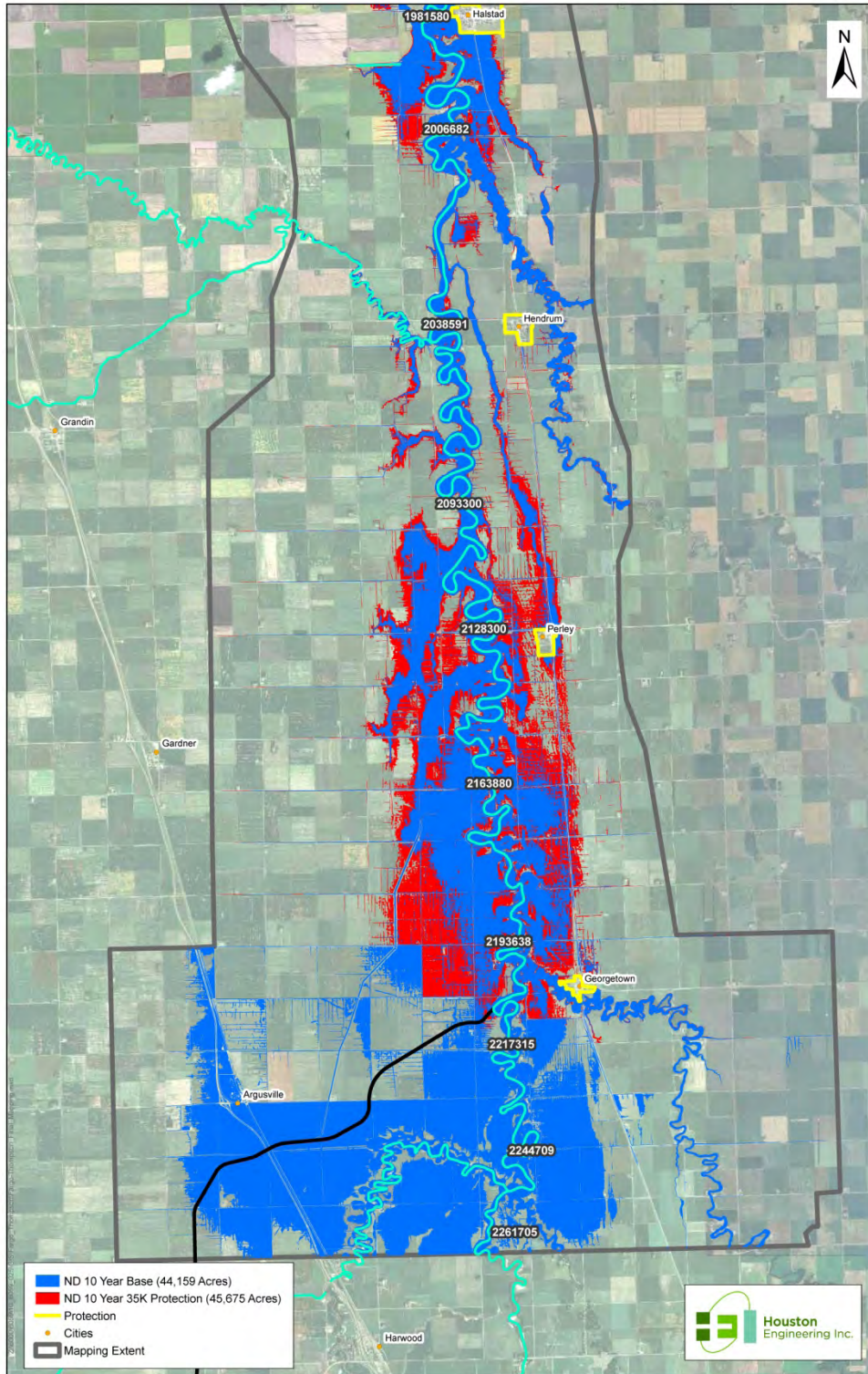
Figure 57 – 10-percent chance event (10-year) downstream to Halstad—existing vs. ND35K
