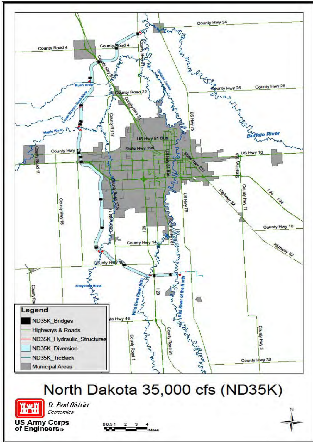
Figure 36- ND35K Diversion Alignment & Features
