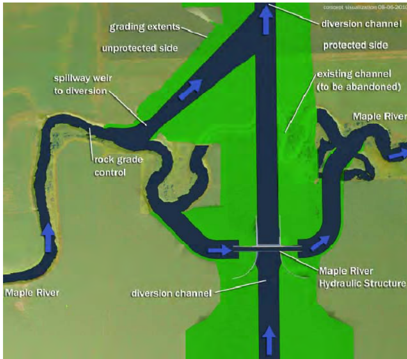
Figure 33 - Maple River crossing conceptual drawing
