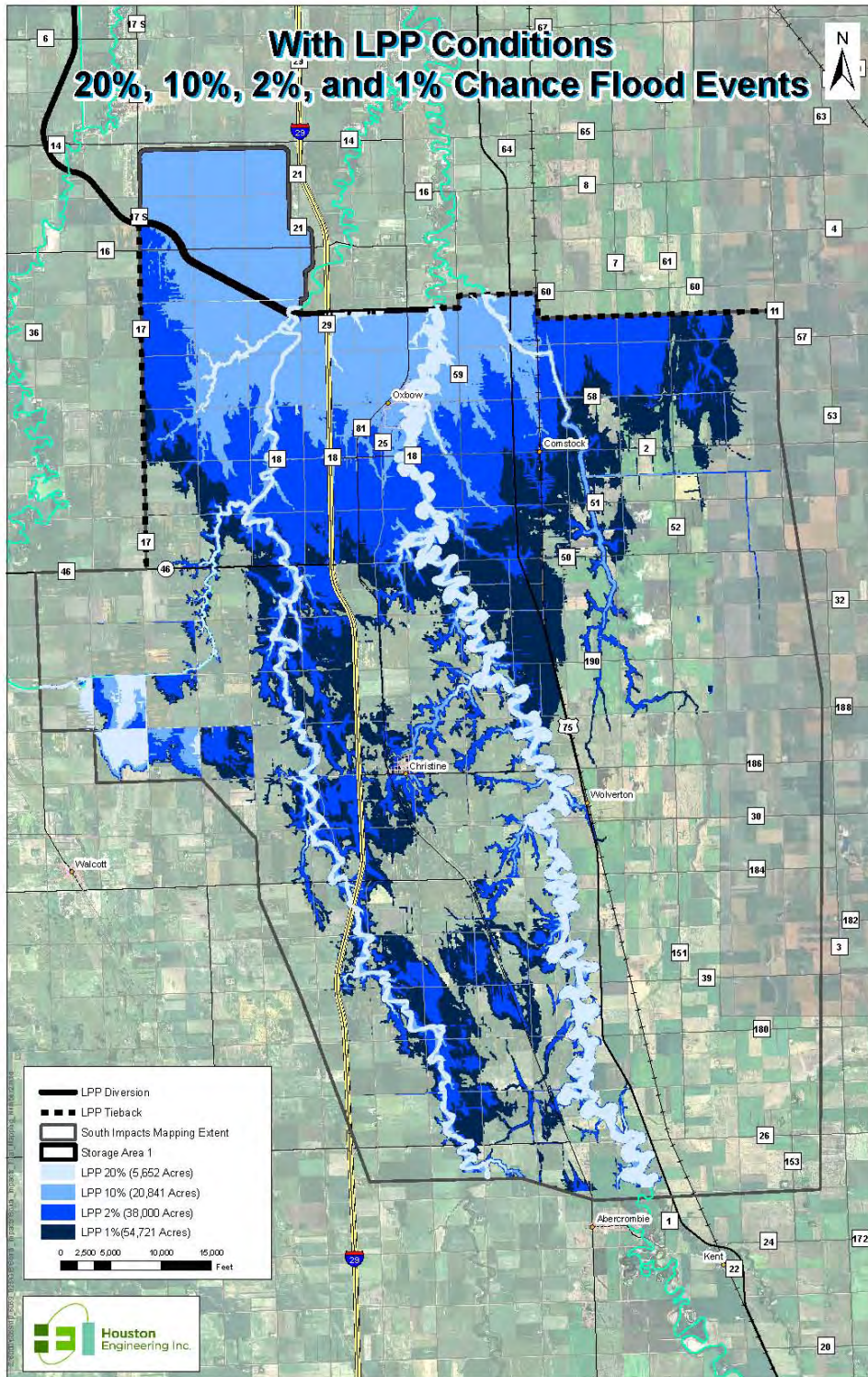
Figure 74 - Upstream staging impacts for the 20 percent, 10 percent, 2 percent, and 1 percent chance events
