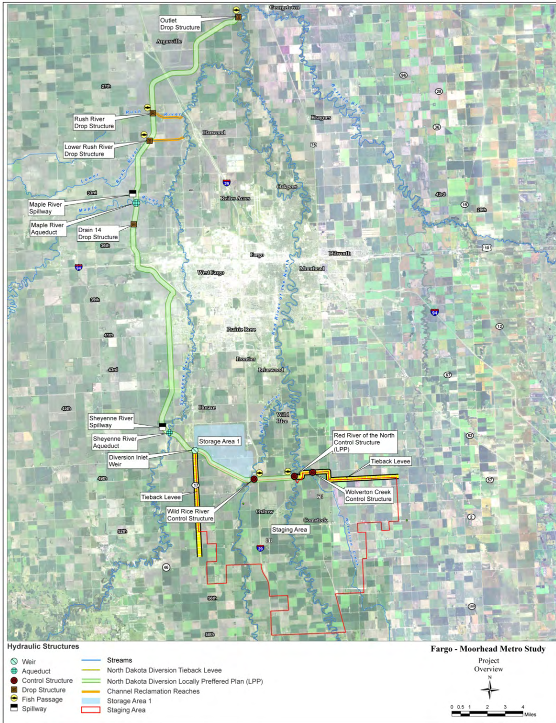
Figure 27 – LPP Diversion Alignment and features
