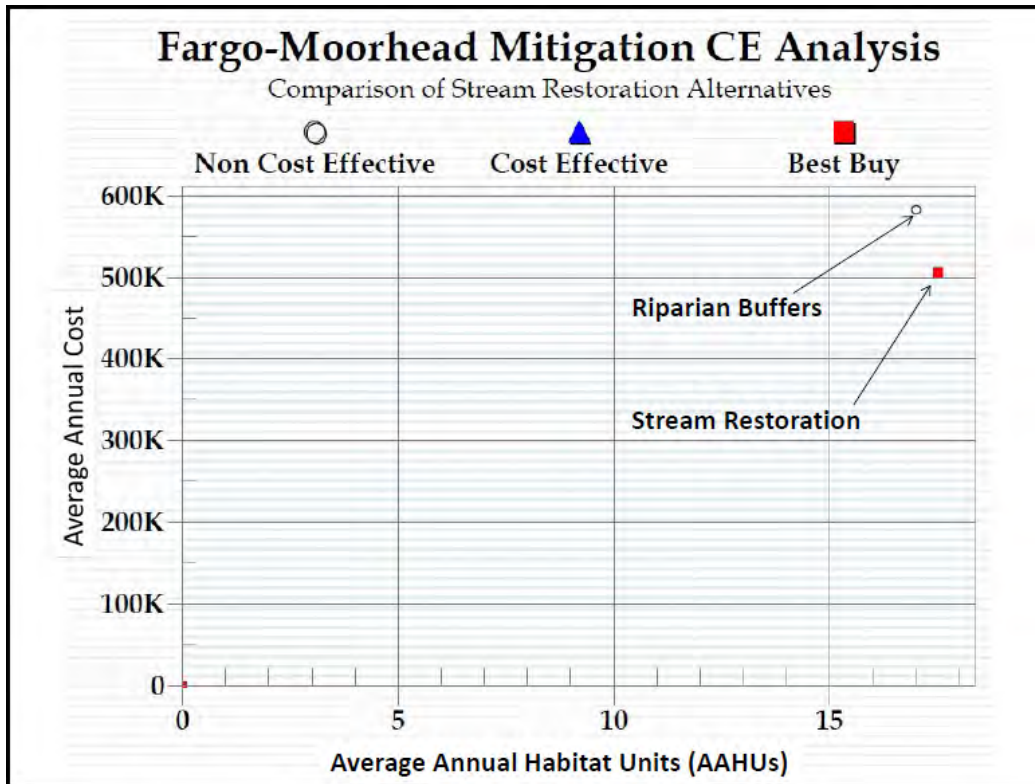
Figure 2 Cost Effectiveness analysis for the two stream restoration alternatives considered for mitigation of aquatic habitat impacts under the Fargo-Moorhead Flood Risk Management Study.
