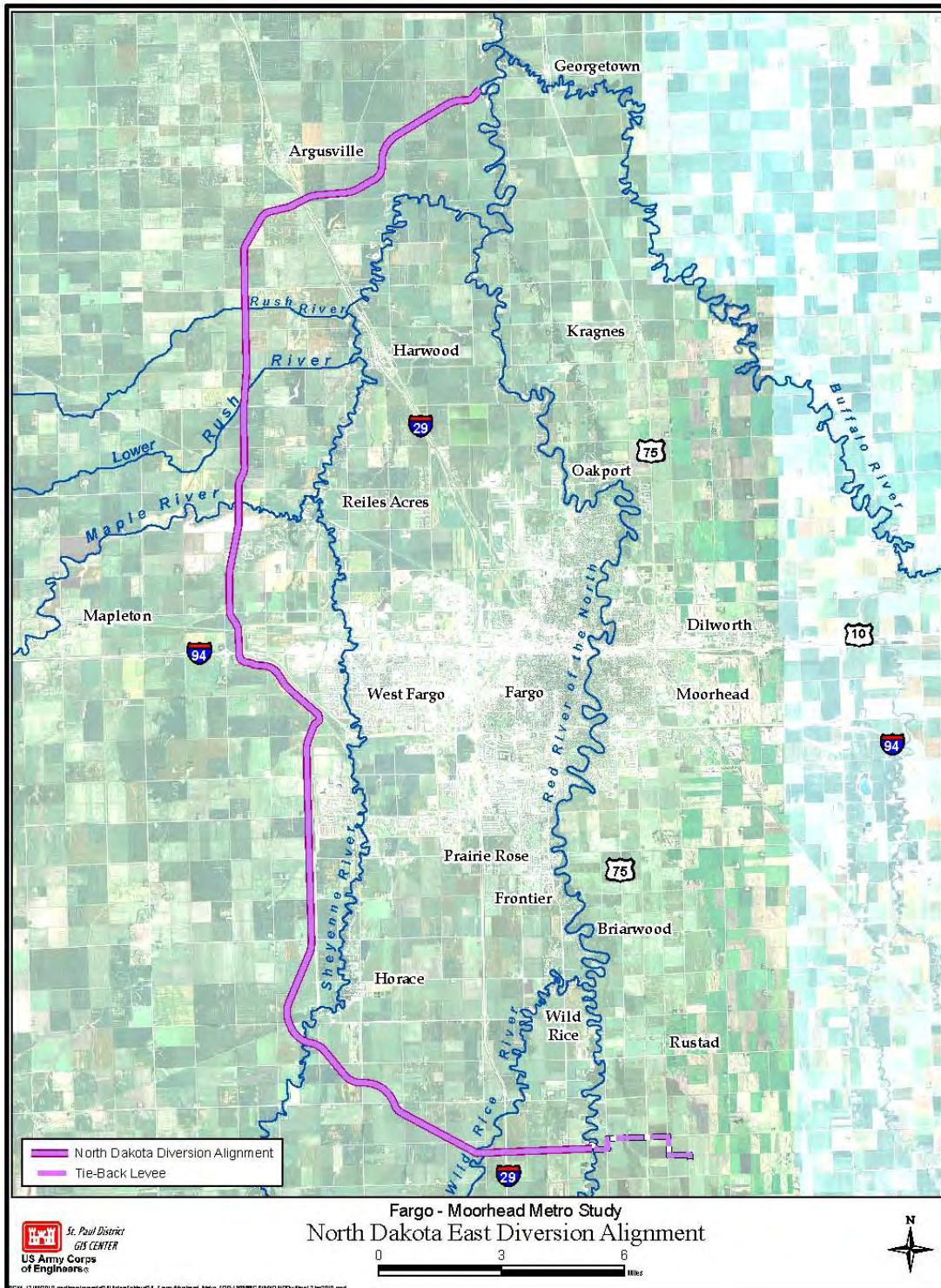
Figure 17 - North Dakota East diversion alignment
