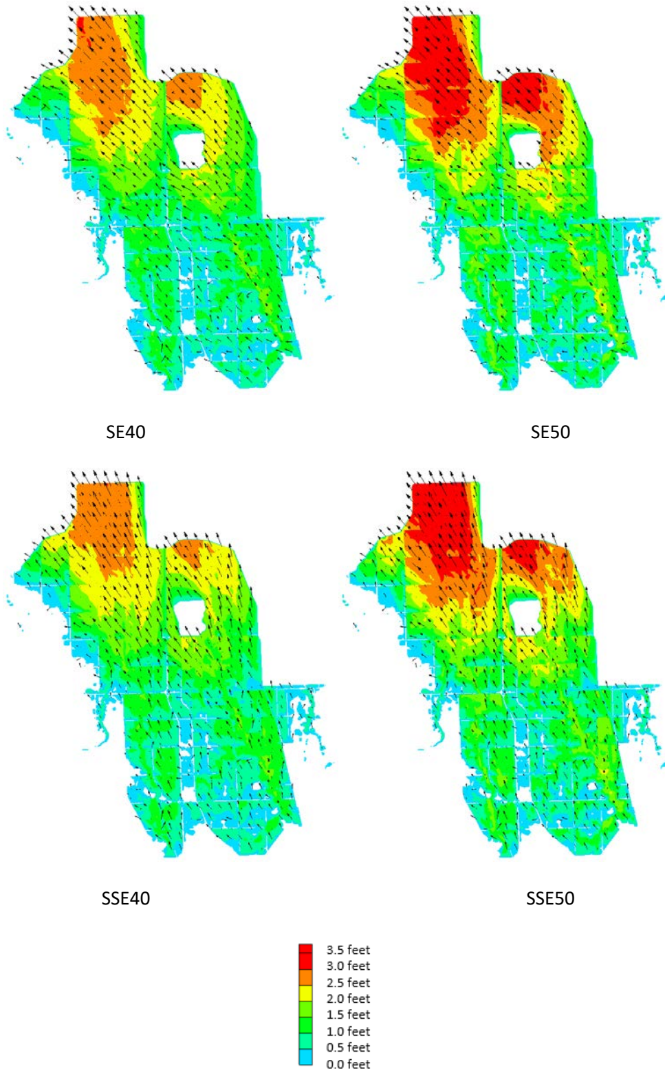
Figure 13: Wave heights in feet for winds from the southeast and south-southeast
