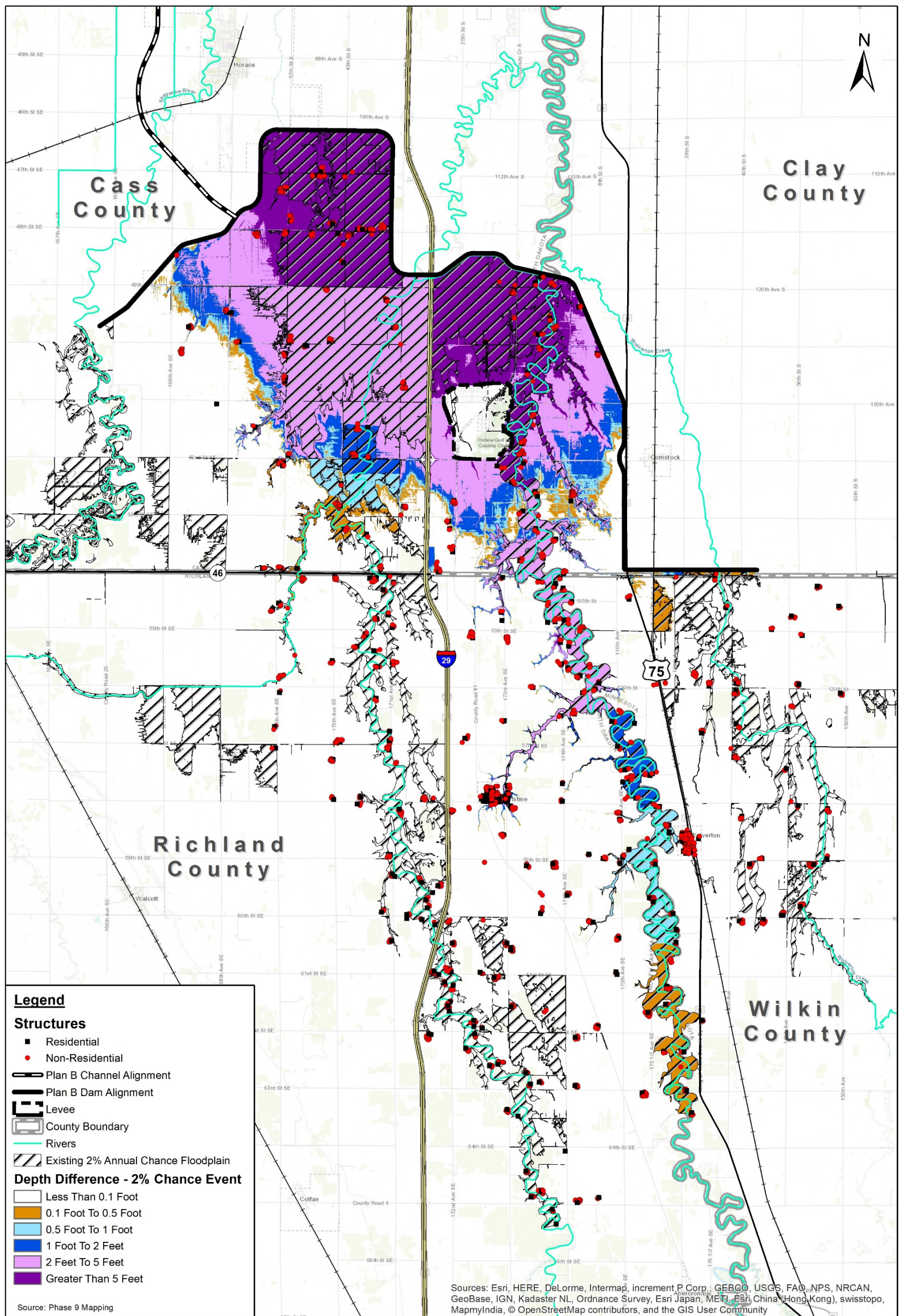
Figure 38: Depth Difference Pool, 2% ACE Event
