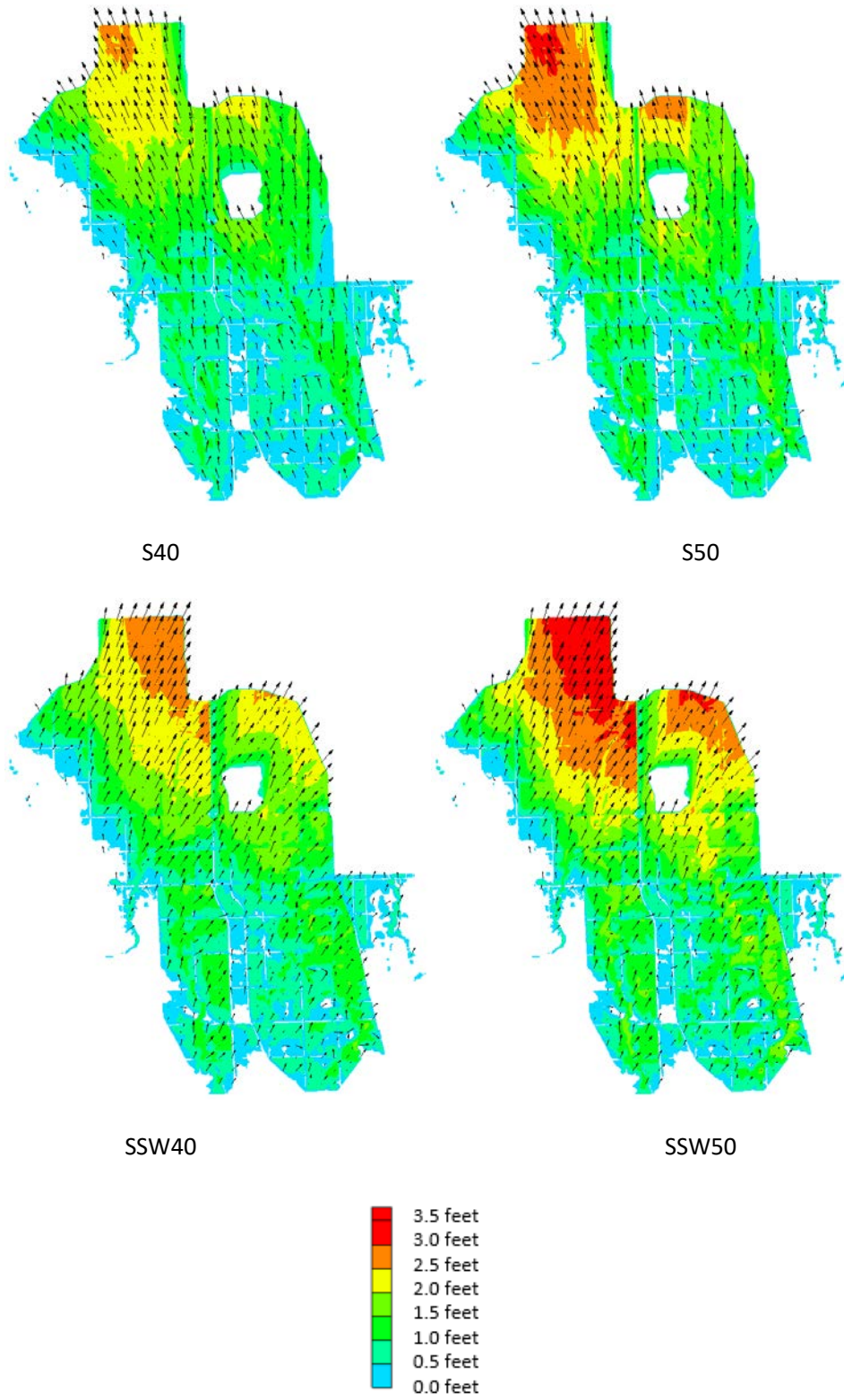
Figure 14: Wave heights in feet for winds from the south and south-southwest
