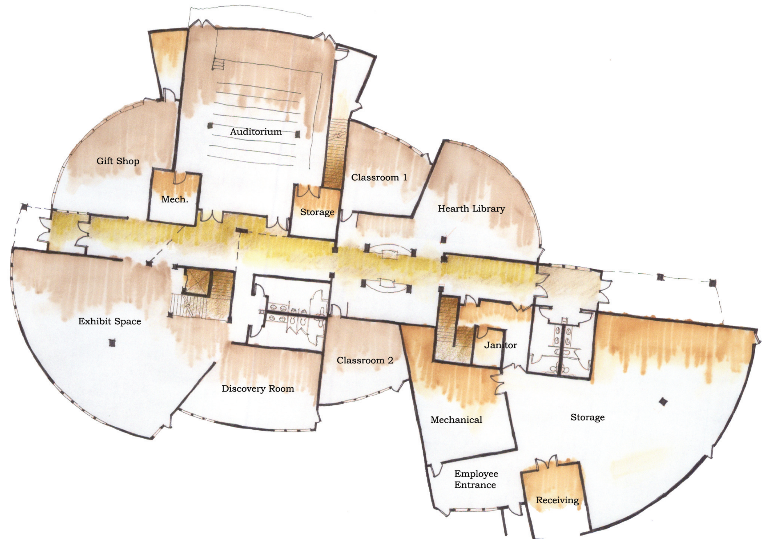
Education Facility Floor 1 1/16" = 1'
