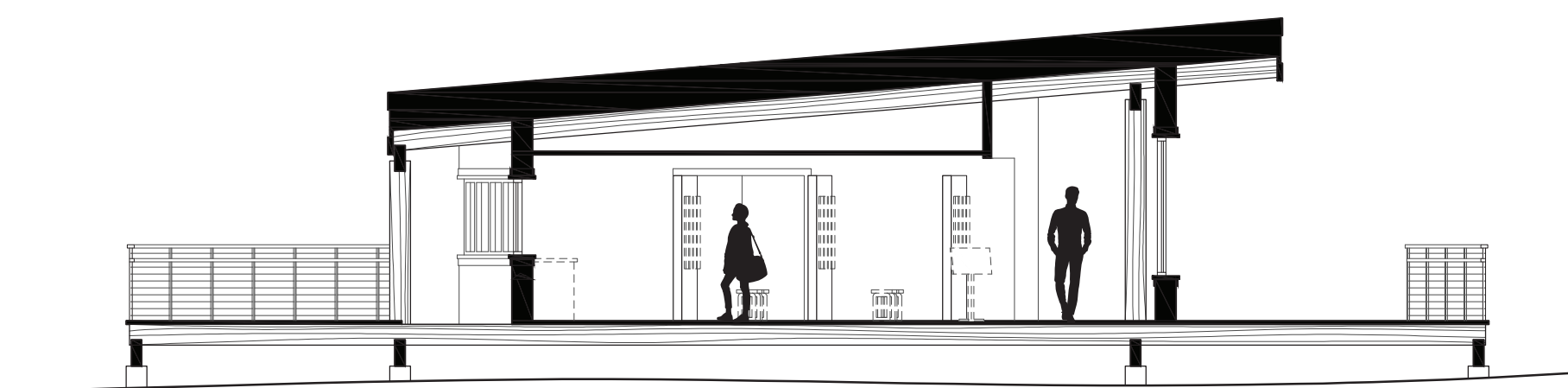
4 History Exhibit Section Cut 1/8" = 1'
