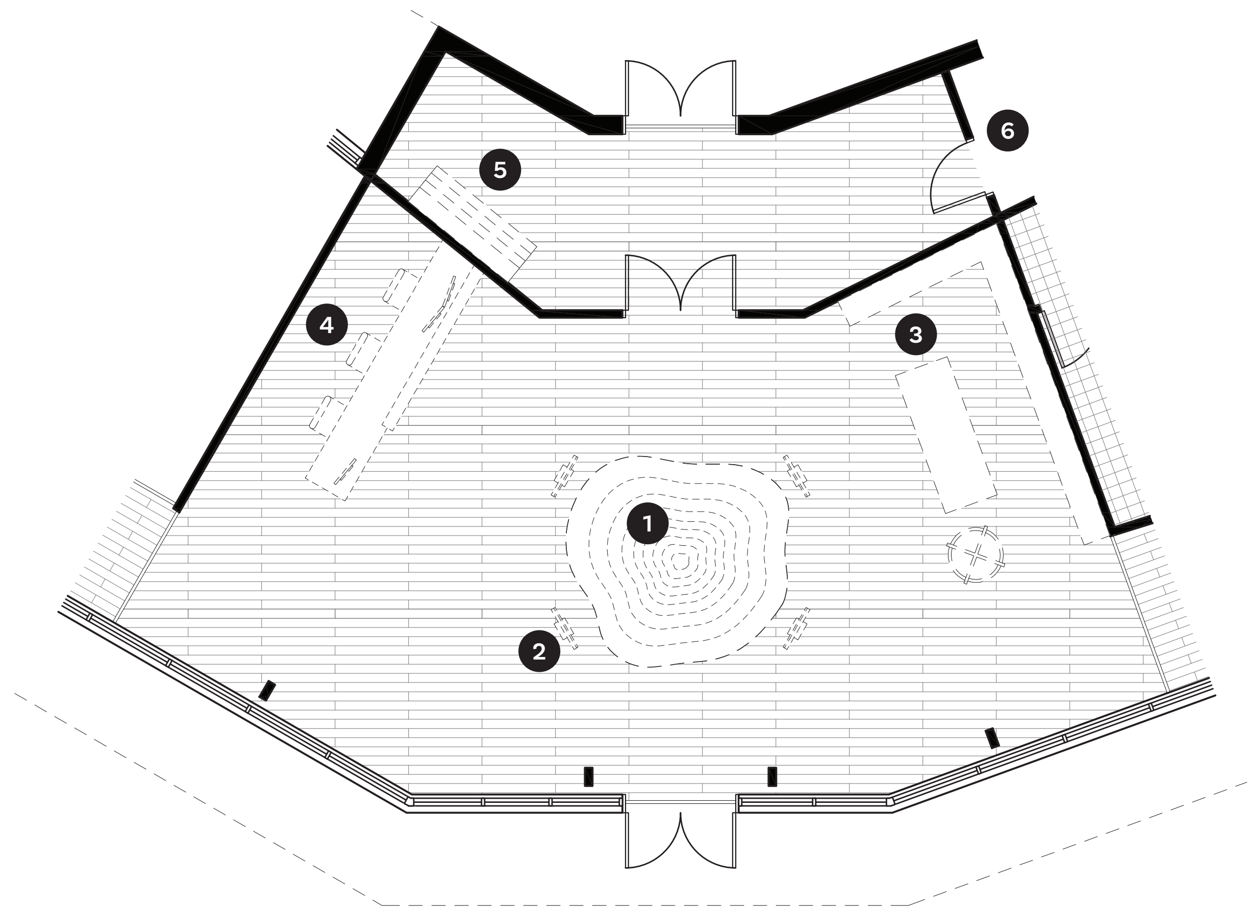
7 Entry/ Lobby Floor Plan 3/16" = 1'
