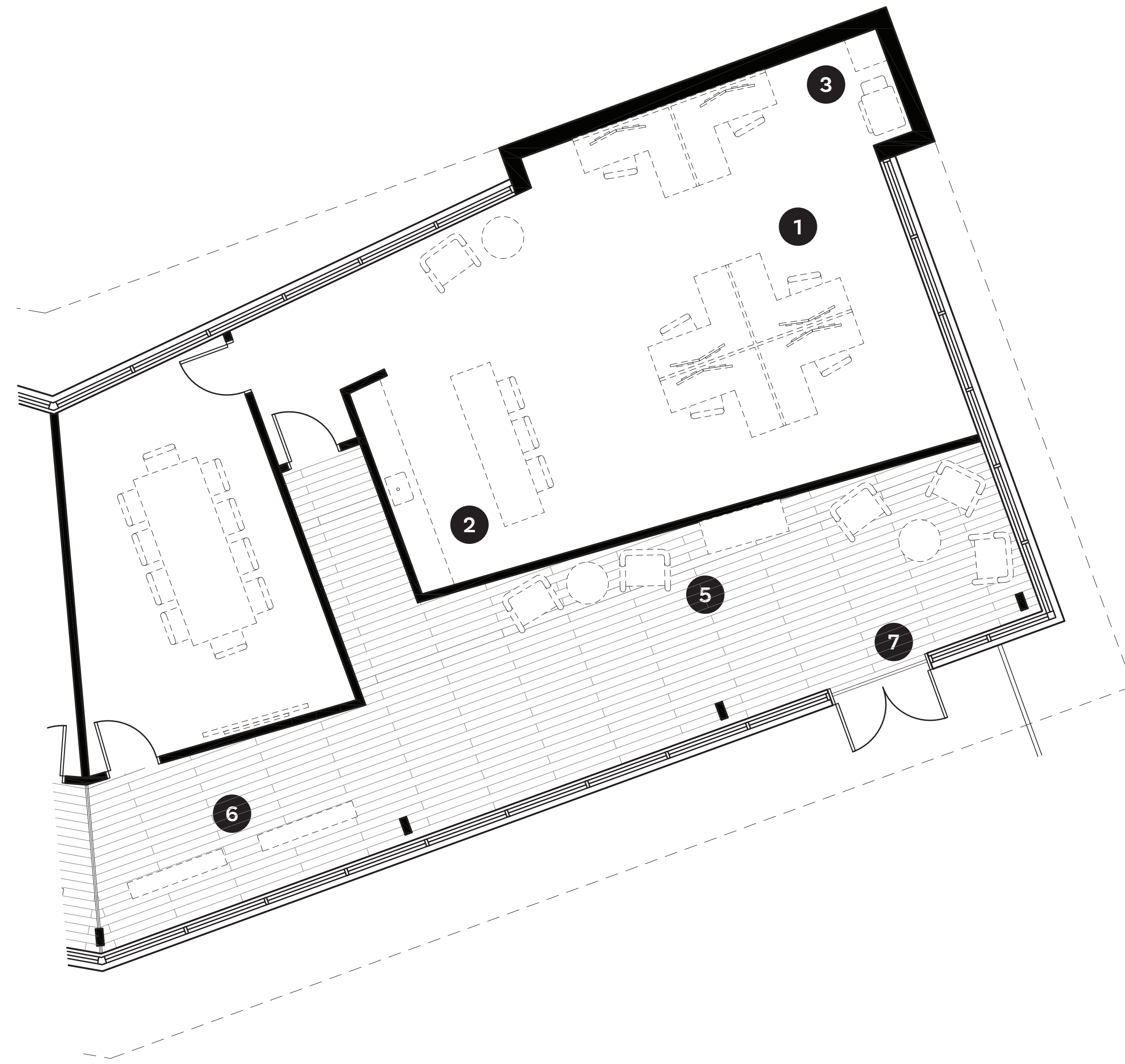
9 Office Area Floor Plan 3/16" = 1'
