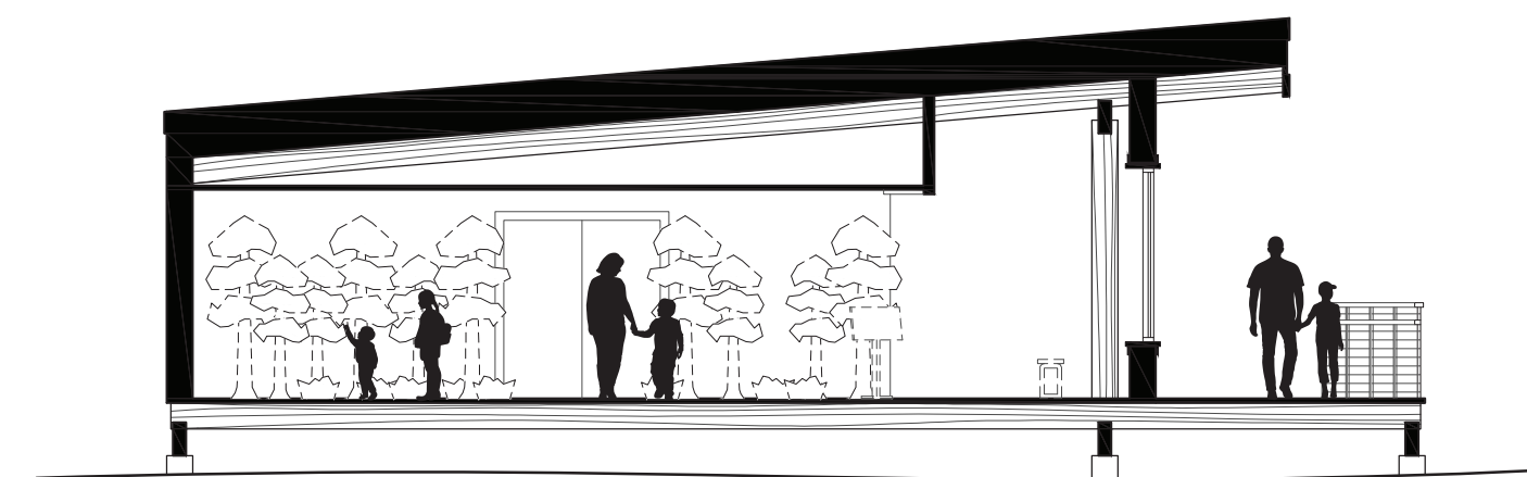
2 Interpretive Exhibit Section Cut 1/8" = 1'
