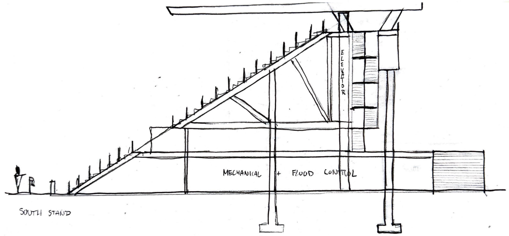
SOUTH STAND SECTION
