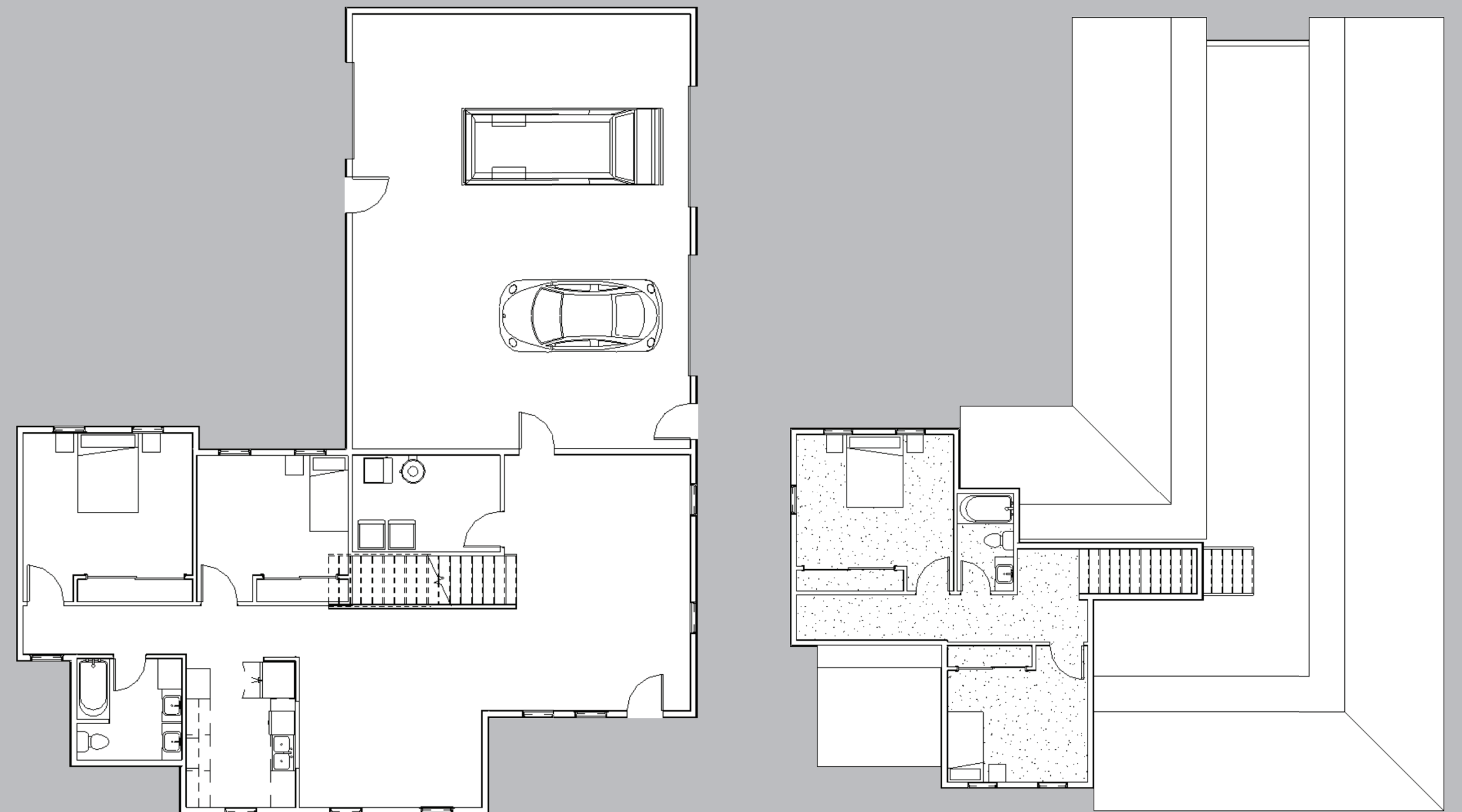
HOUSE 2 ADDITION - LEVEL 1 & 2 FLOOR PLANS
