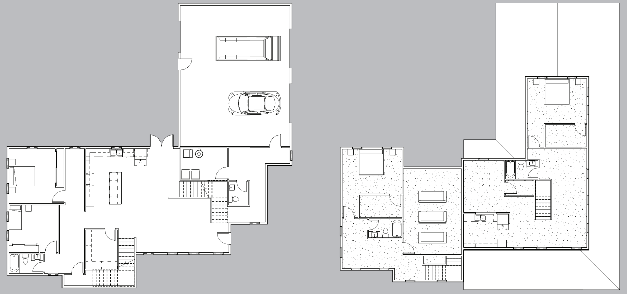
HOUSE 5 ADDITION - LEVEL 1 & 2 FLOOR PLANS
