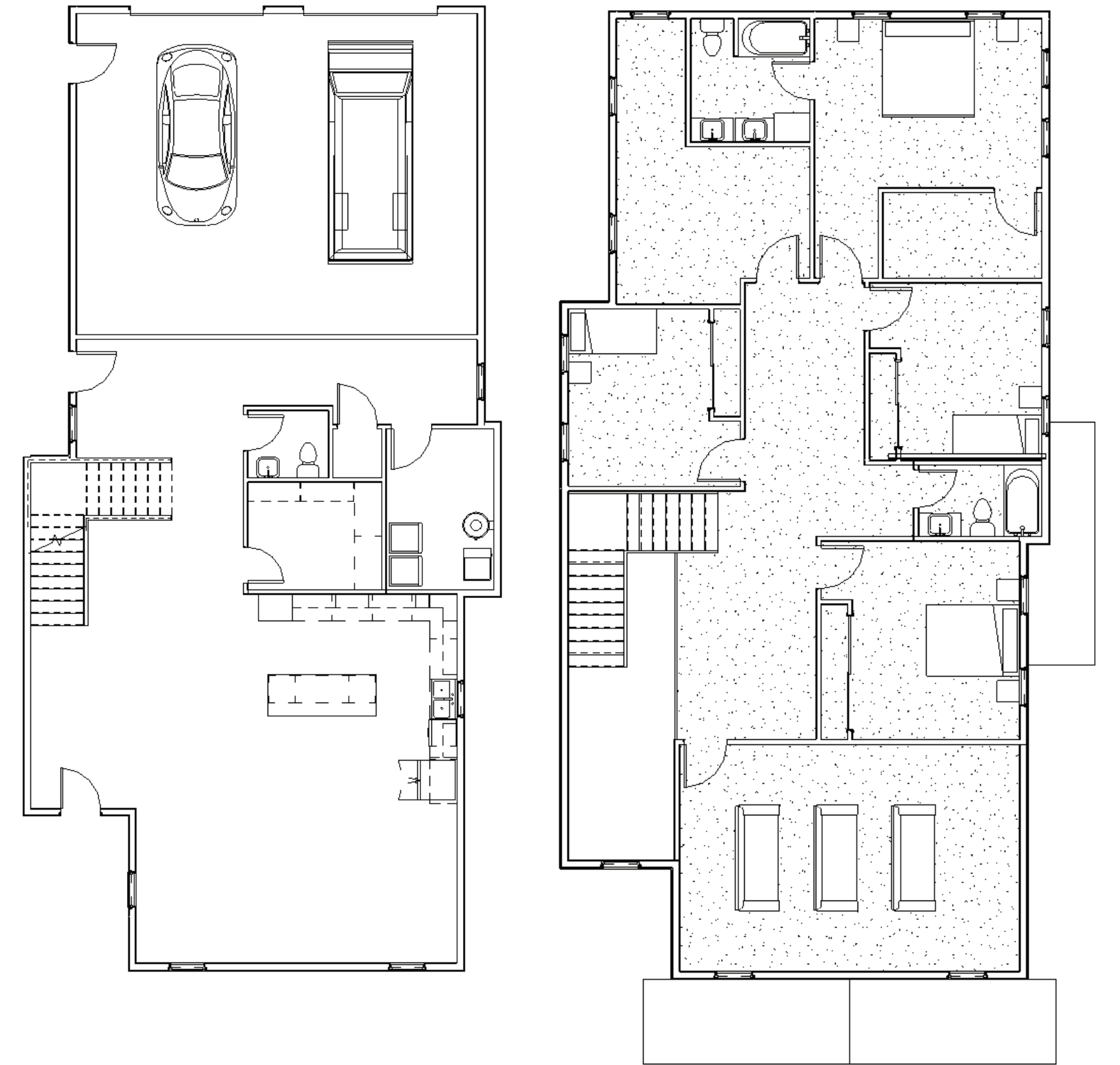
HOUSE 3 - LEVEL 1 & 2 FLOOR PLANS
