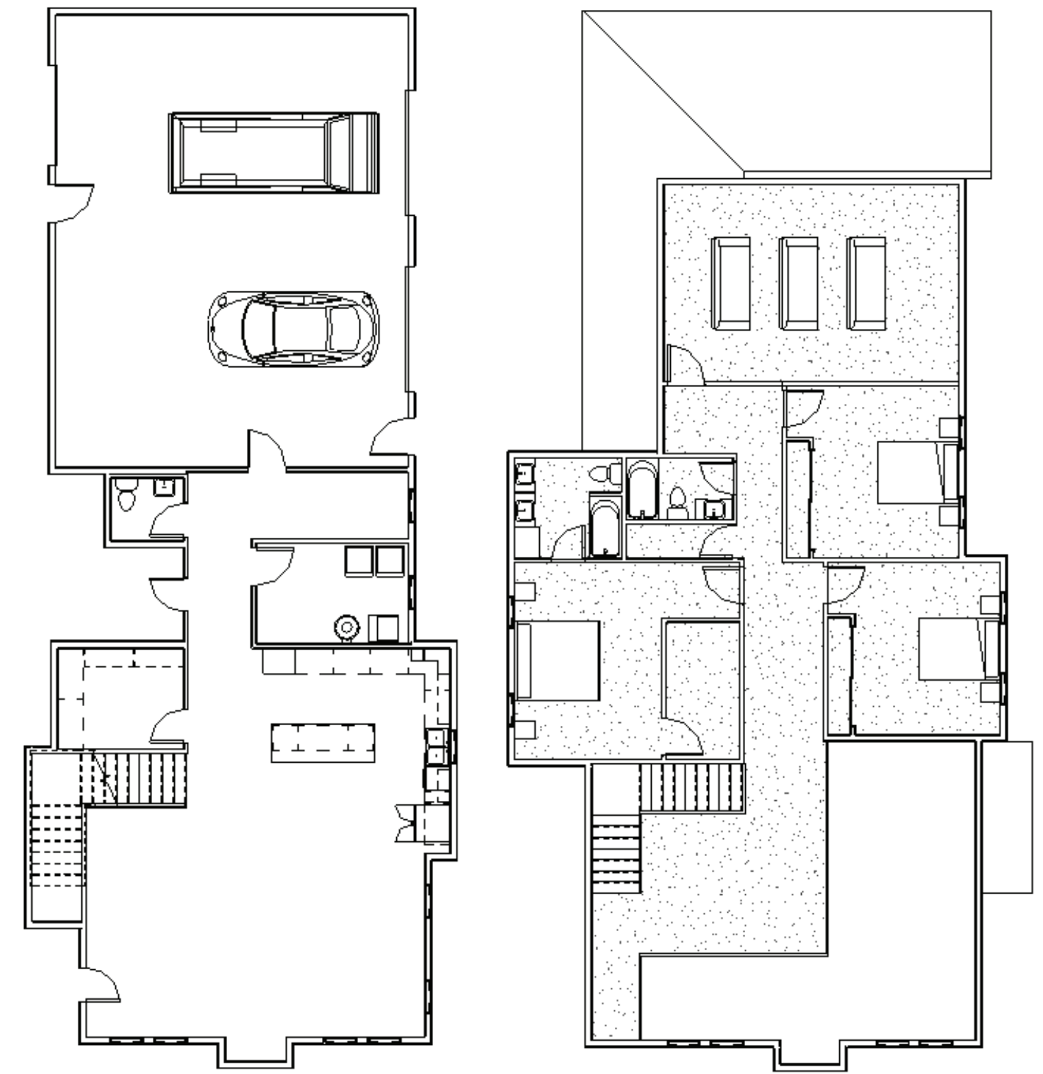
HOUSE 1 – LEVEL 1 & 2 FLOOR PLANS
