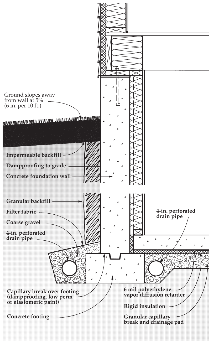
Figure 7. Foundation drainage system.
