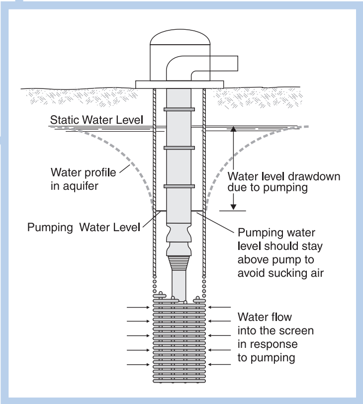
Figure 2. Side view of pumping irrigation well.
