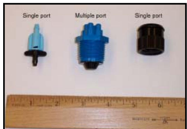
Figure 4. Bubbler emitters of different shapes with single and multiport exits.
