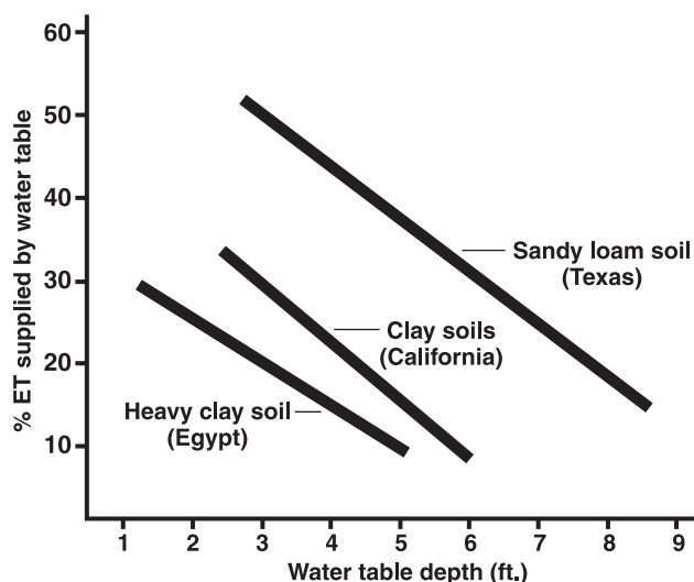
Figure 7. Evapotranspiration supplied by a saline water table as affected by water table depth. (Gismer and Gates, 1988).
