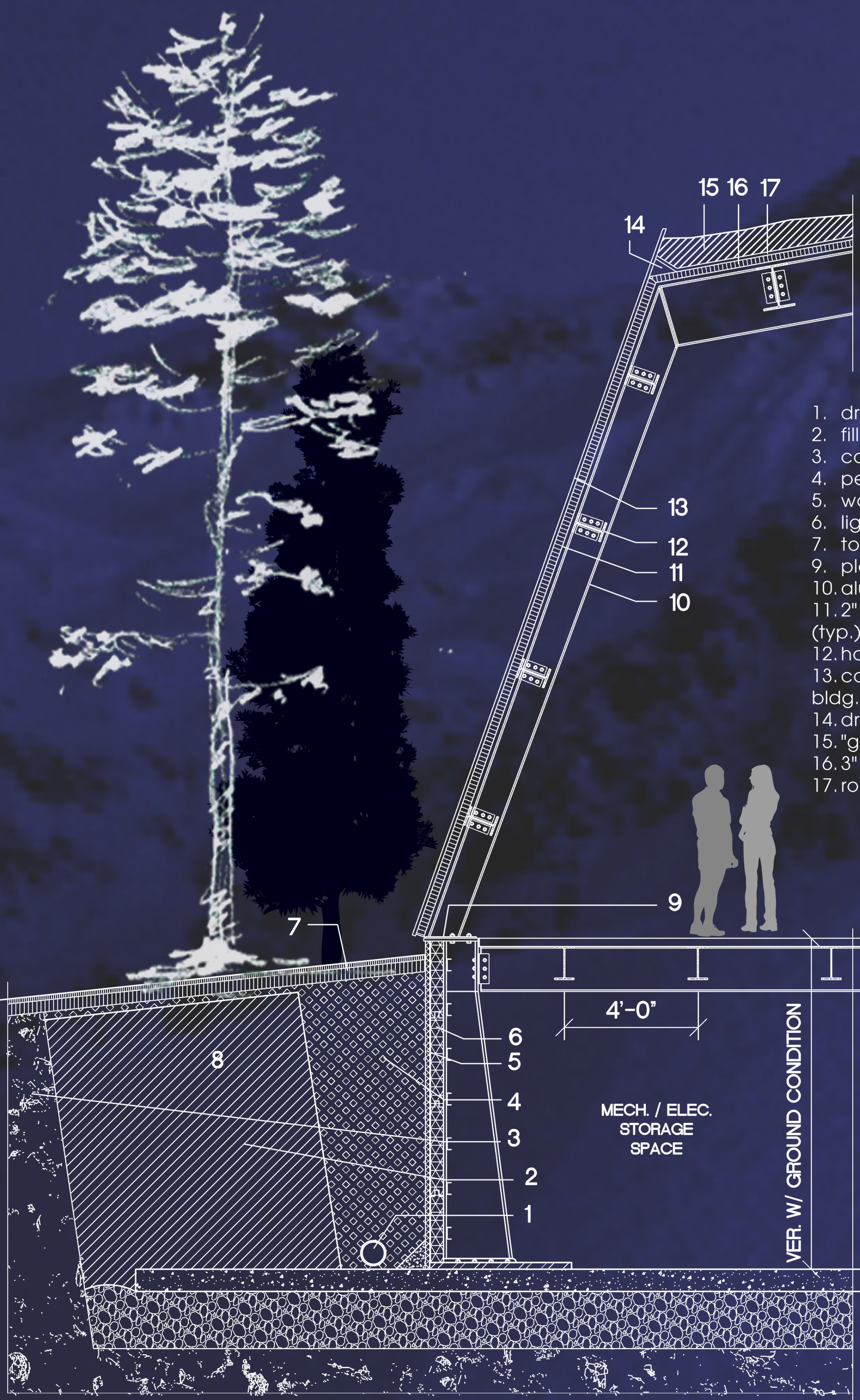
typ. sect. upper station
