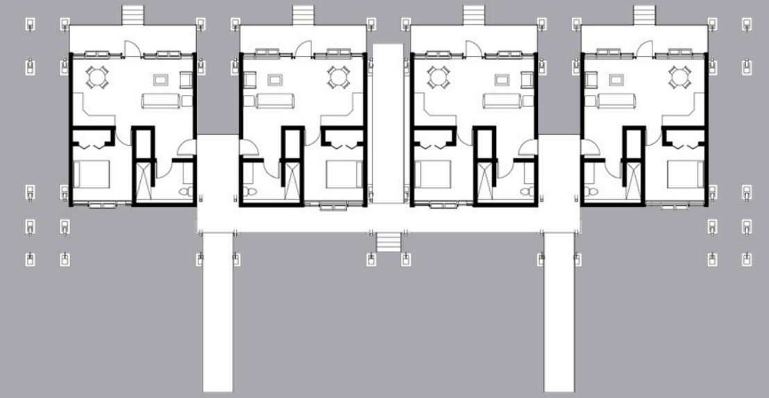
Assisted Living Floor Plan
