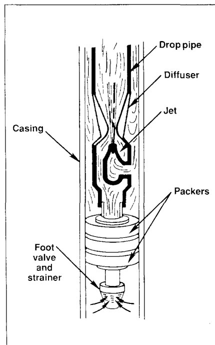
Figure 2. Packer-type Jet Used For Small Wells (2-4 inch).
