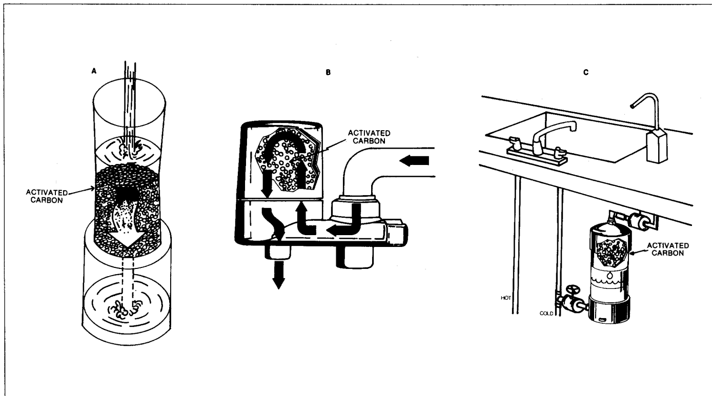
Figure 2. The three types of activated carbon filtration units are: A) pour-through; B) faucet-mounted; and C) high-volume.
