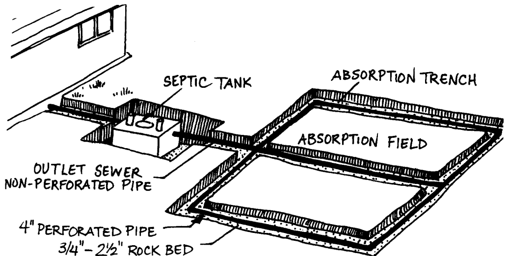
Figure 1. Typical septic tank and drain field.
